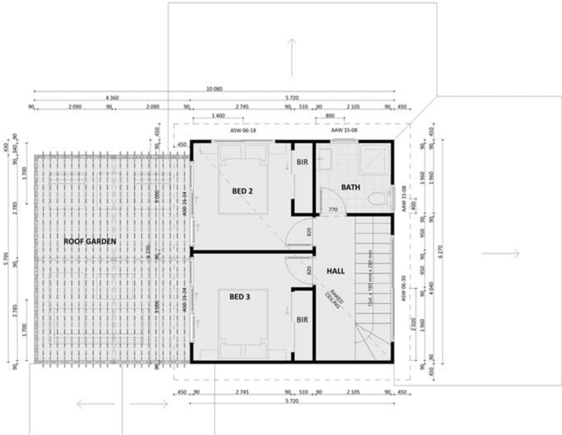
FLOORPLAN_DIMENSION_FIRSTFLOOR_DESIGN_1311
