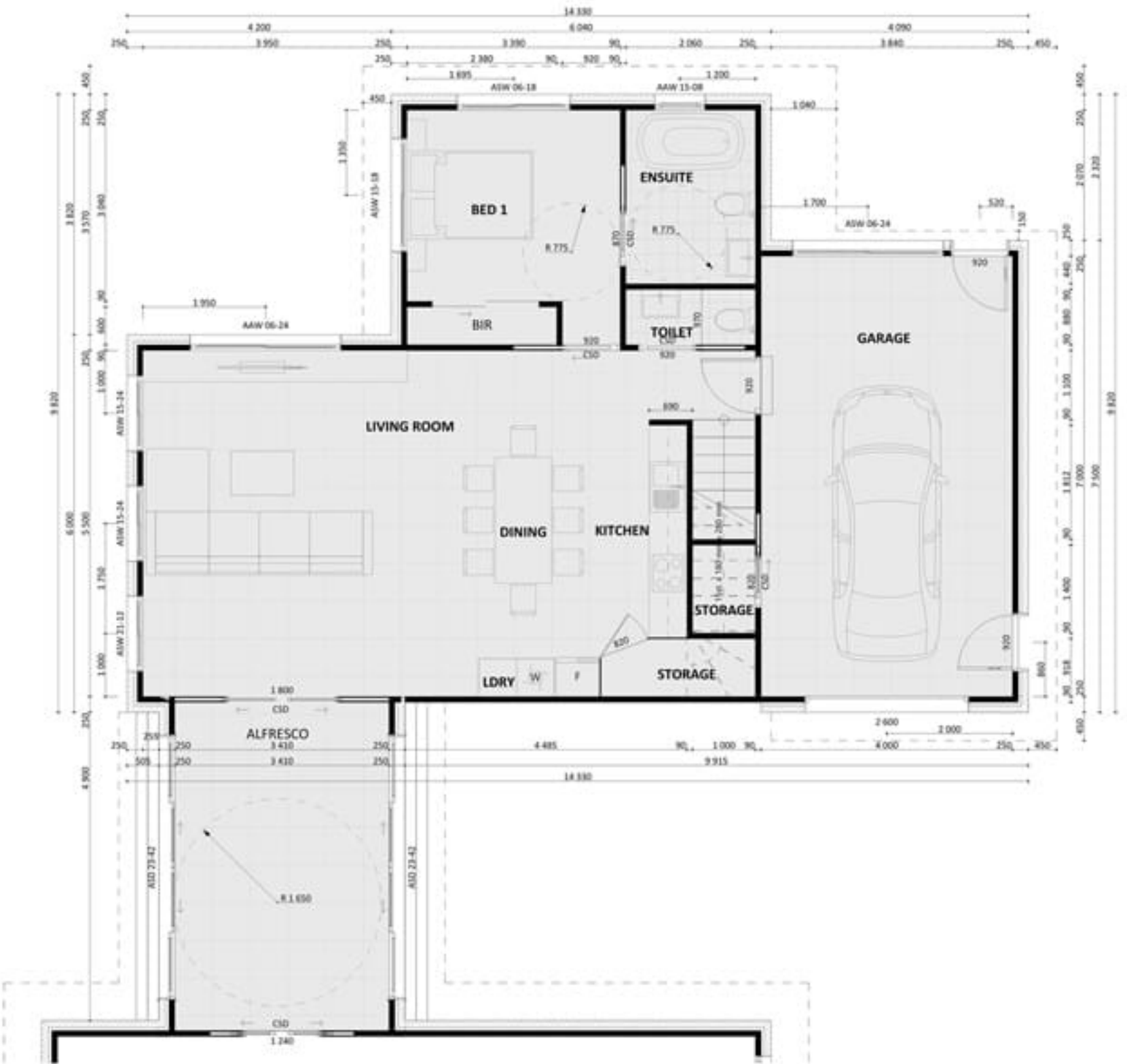
FLOORPLAN_DIMENSION_GROUND FLOOR DESIGN_1311
