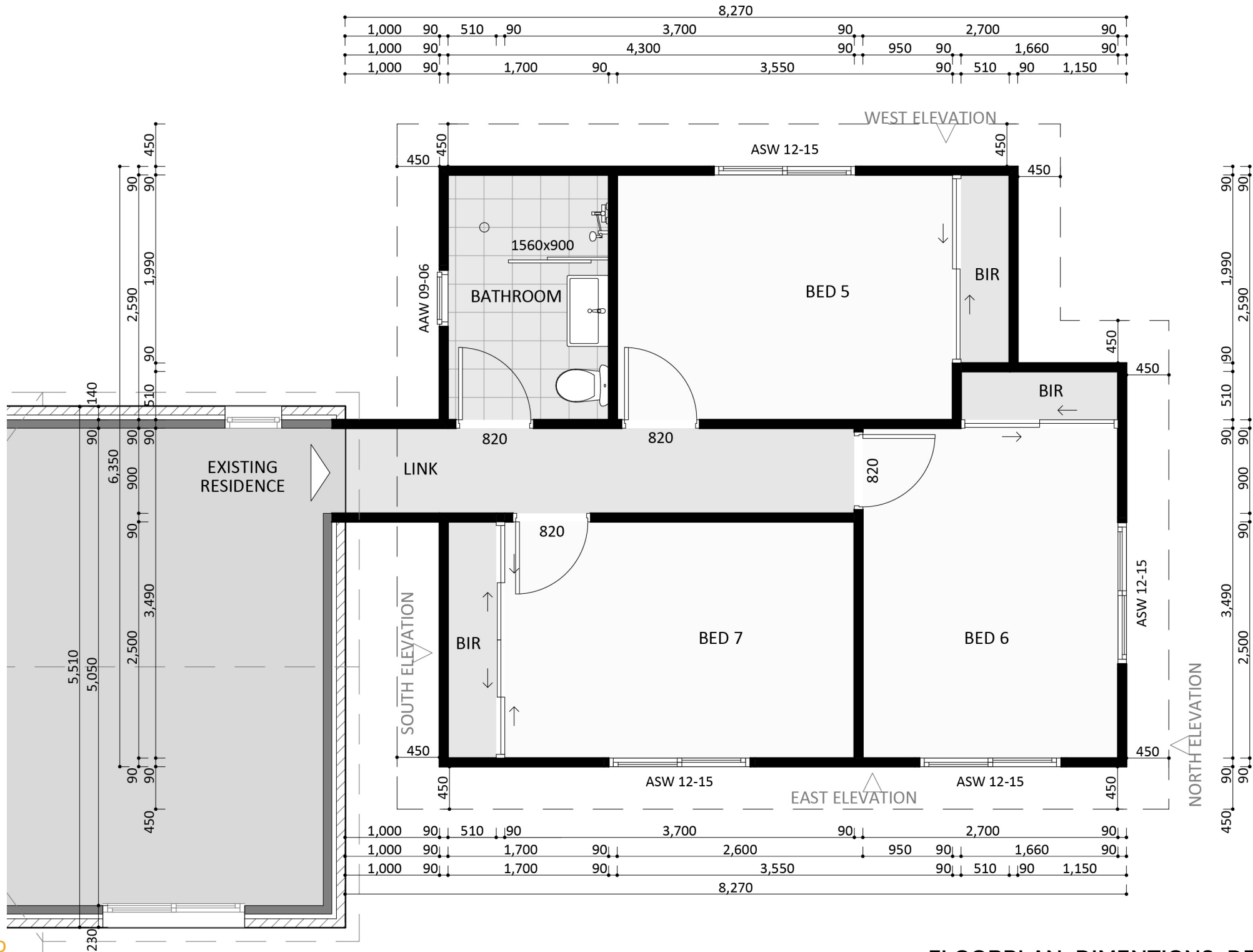
FLOORPLAN_DIMENTIONS_DESIGN_1300
