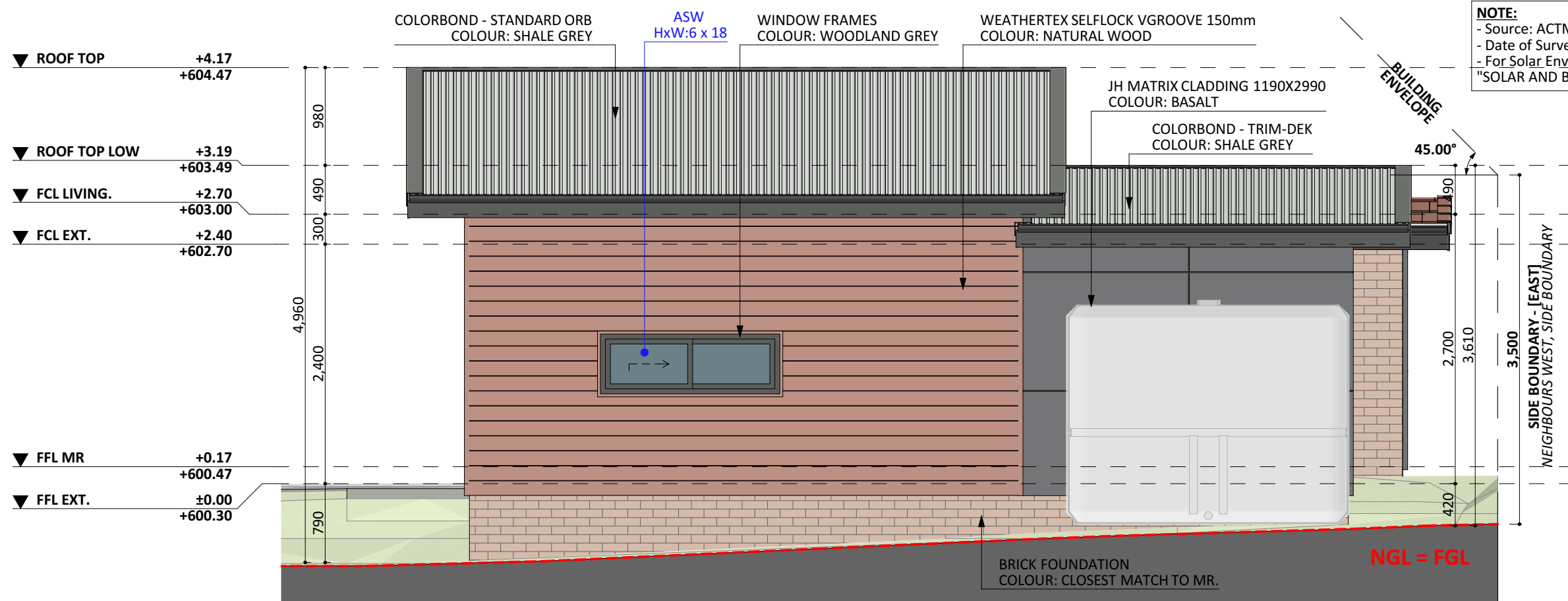
SOUTH ELEV. - EXT.
