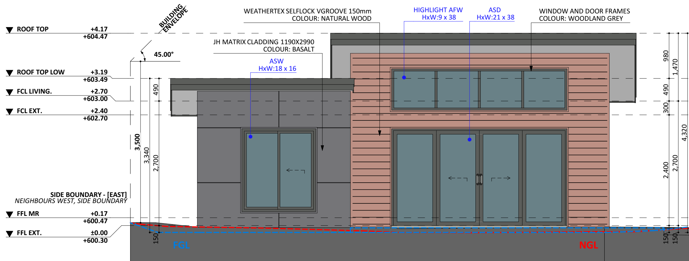
NORTH ELEV. - EXT.
