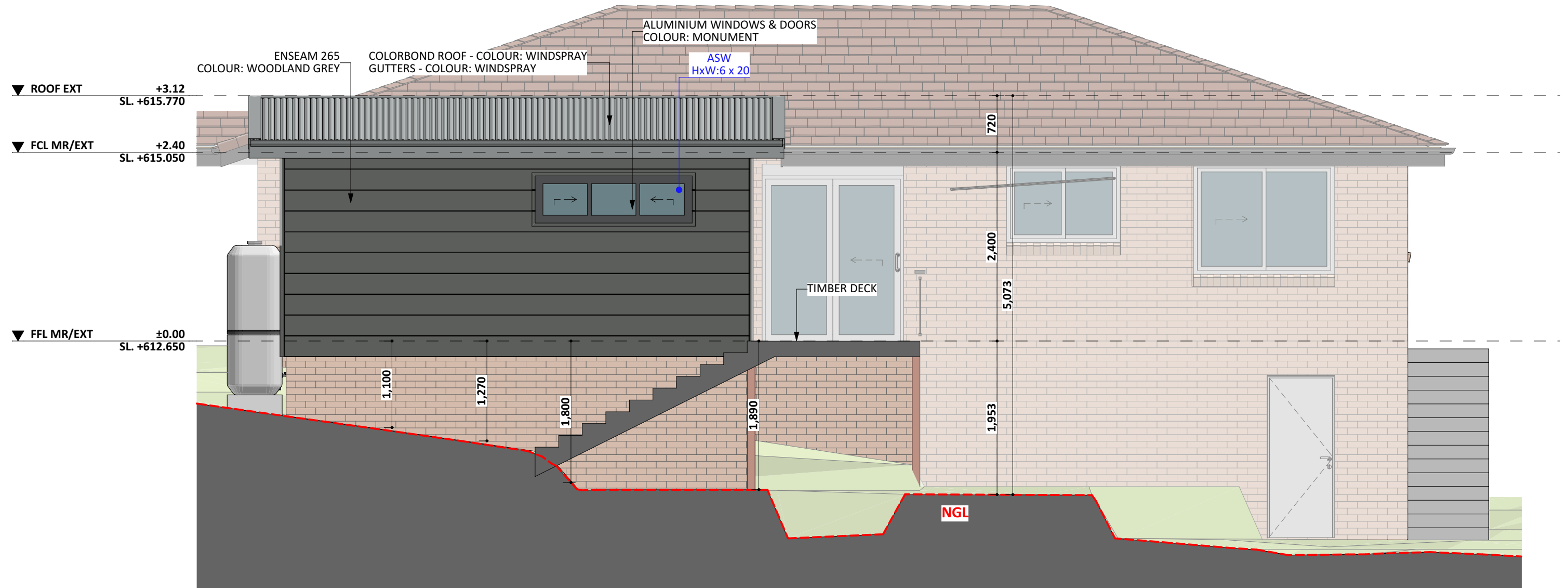
SOUTH ELEV.
