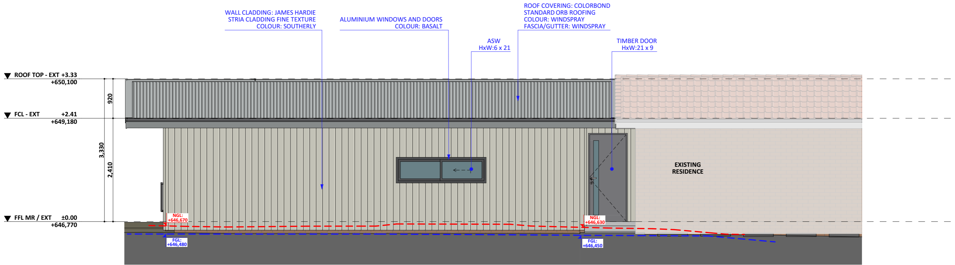
E4 ————— SOUTH-WEST ELEV. 1:55
