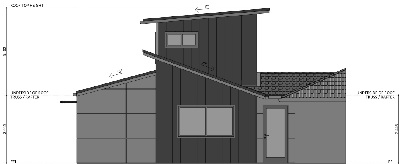
ELEVATION 03
