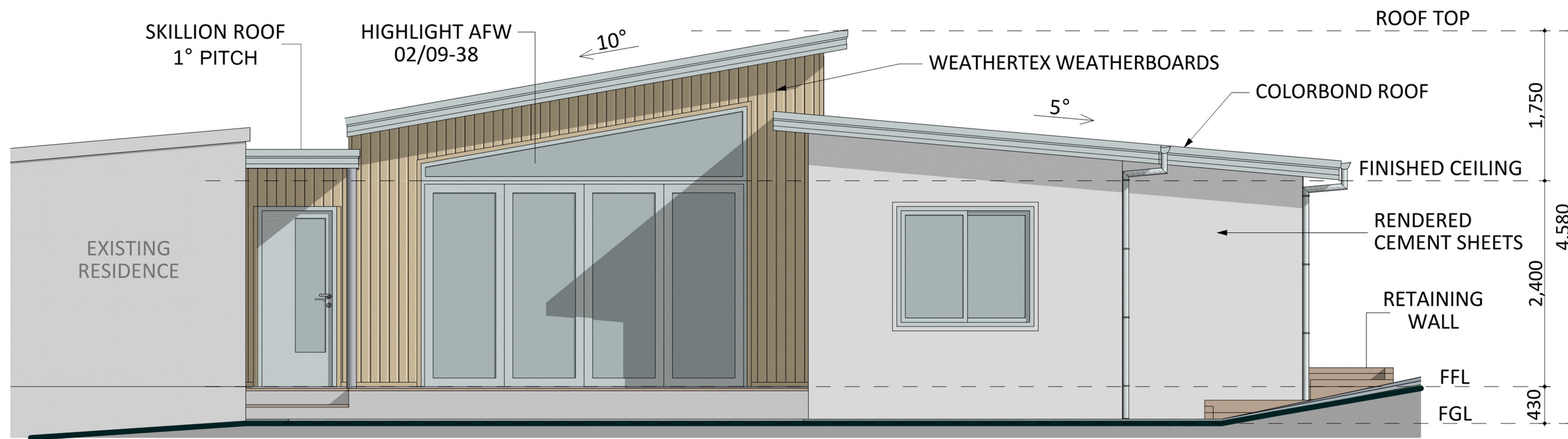
SOUTH ELEVATION
