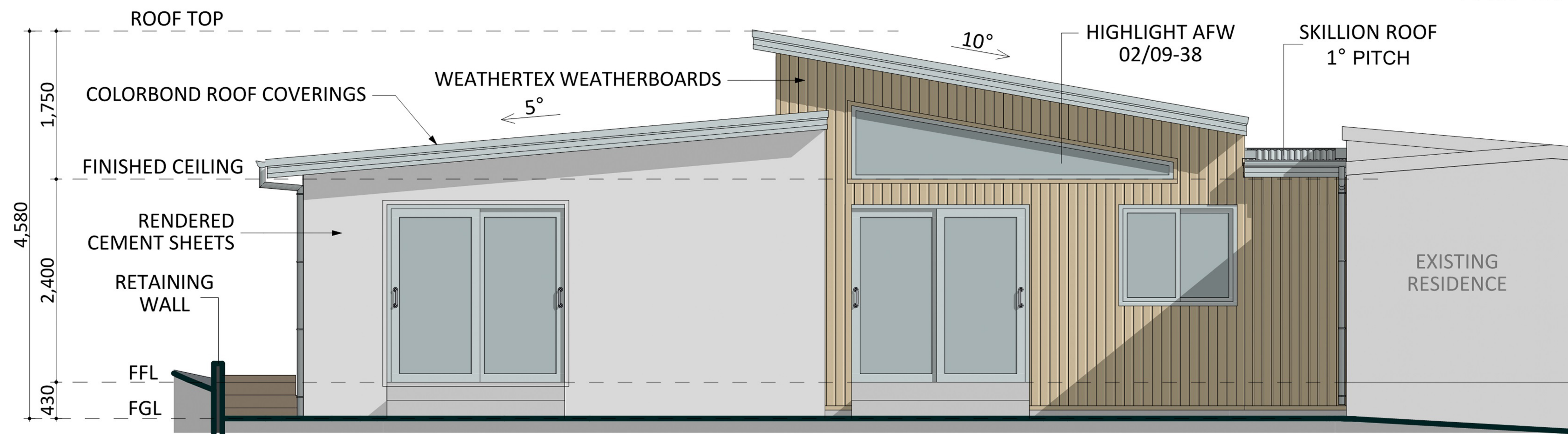
NORTH ELEVATION
