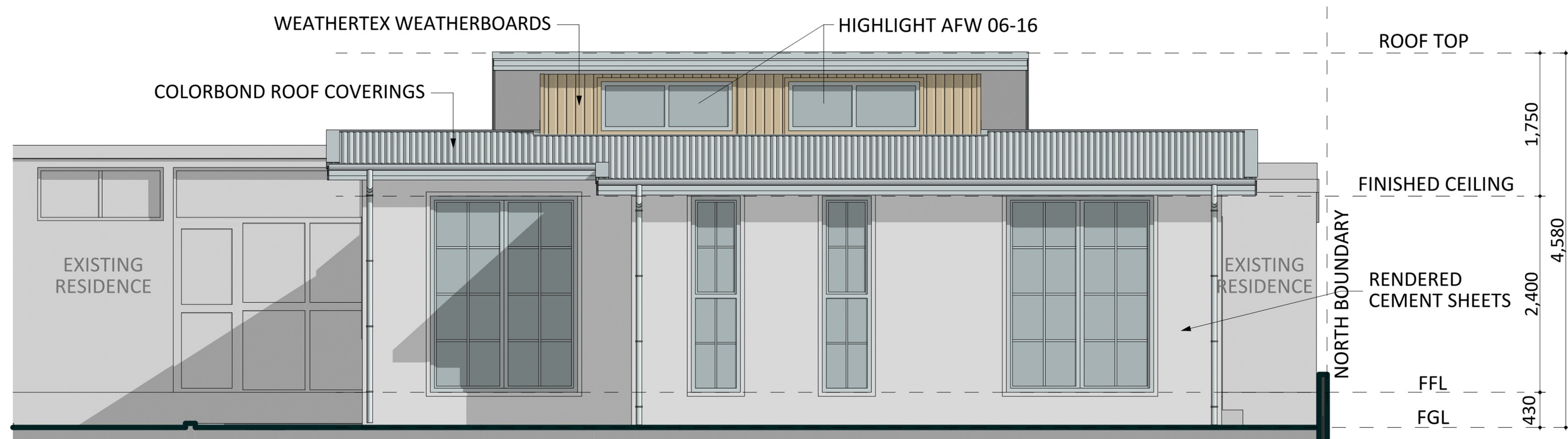
EAST ELEVATION
