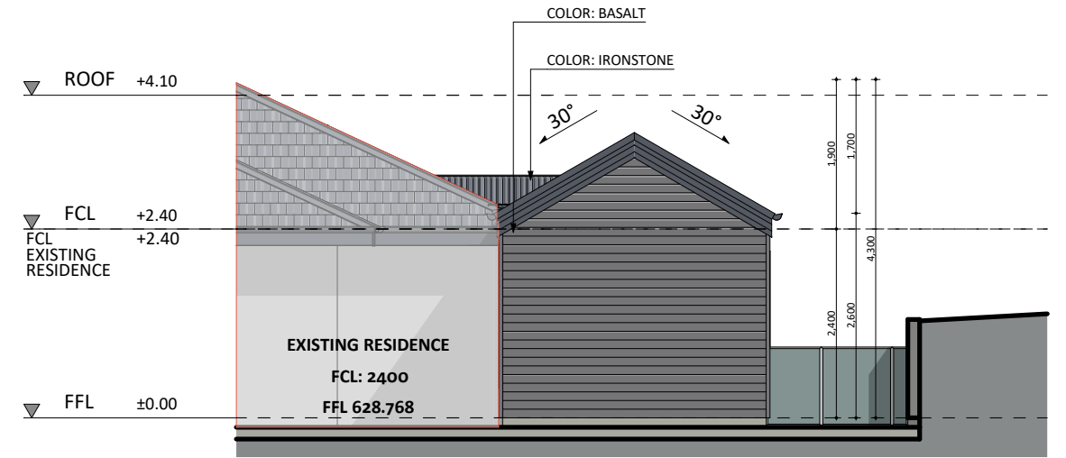
SOUTH-WEST ELEVATION
