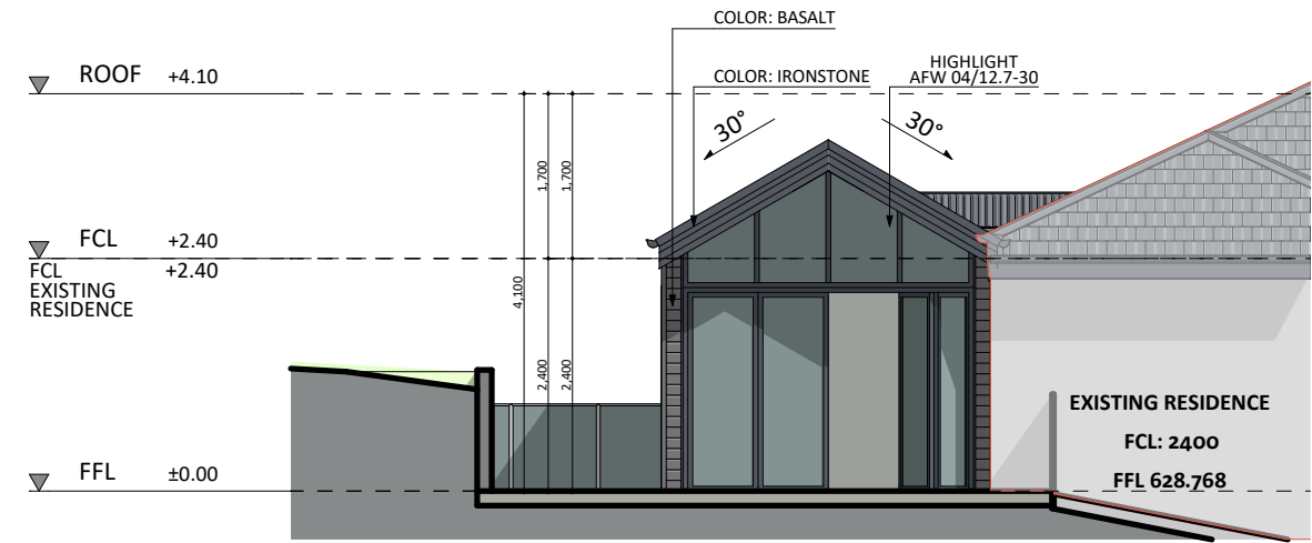
NORTH-EAST ELEVATION
