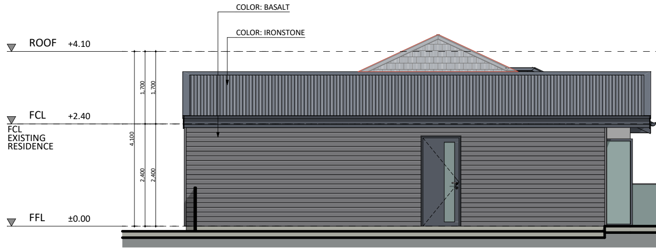
SOUTH-EAST - ELEVATION
