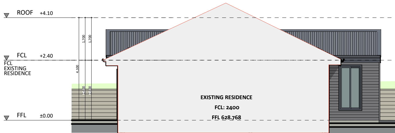
NORTH-WEST ELEVATION
