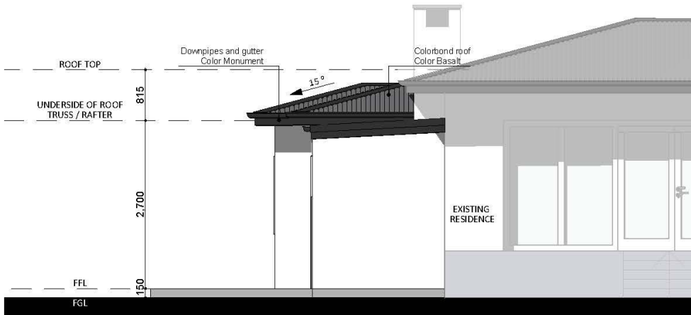
WEST ELEVATION
