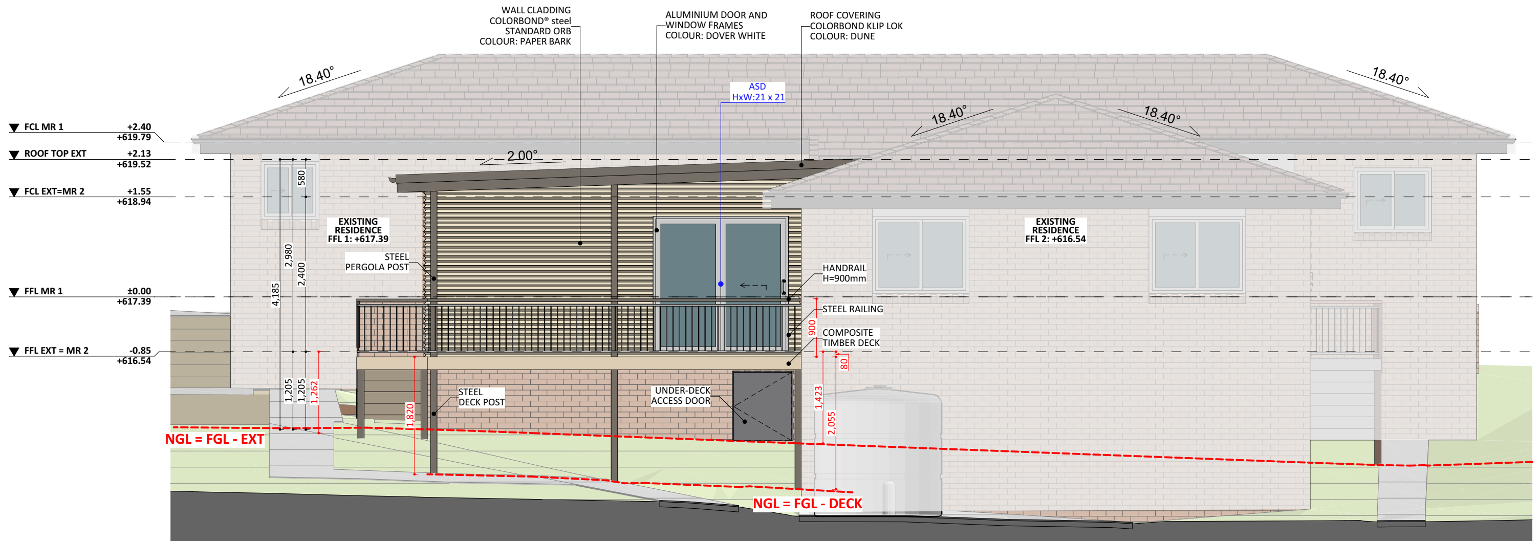
SOUTH ELEV.
