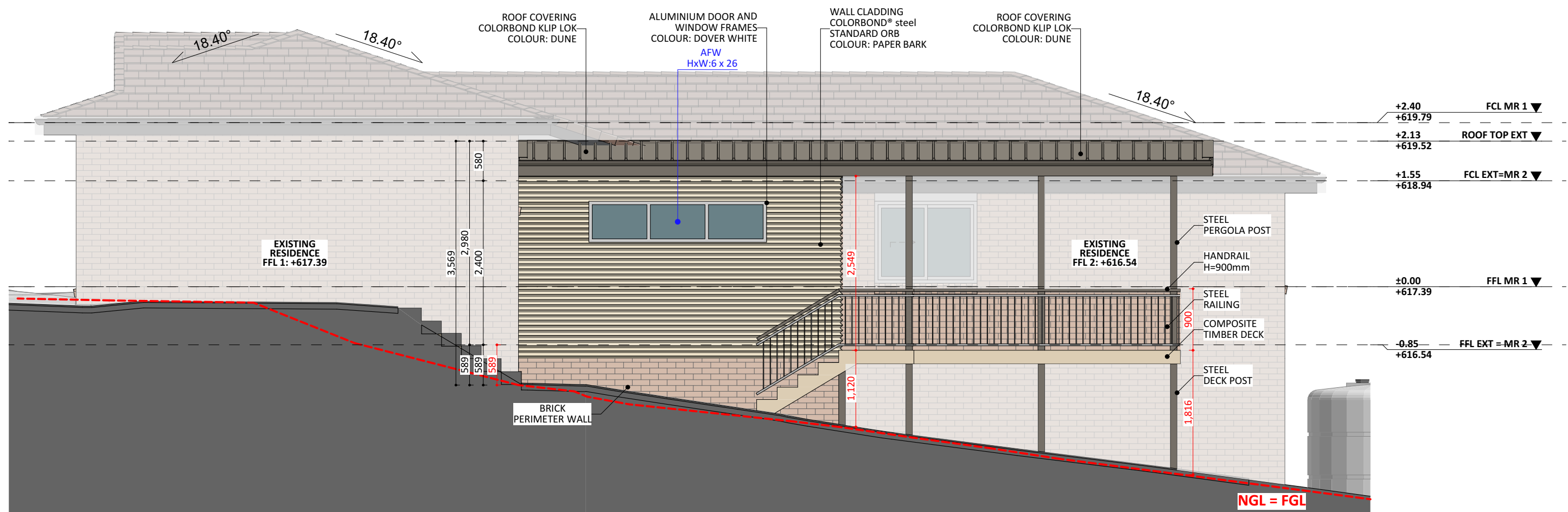
WEST ELEV.
