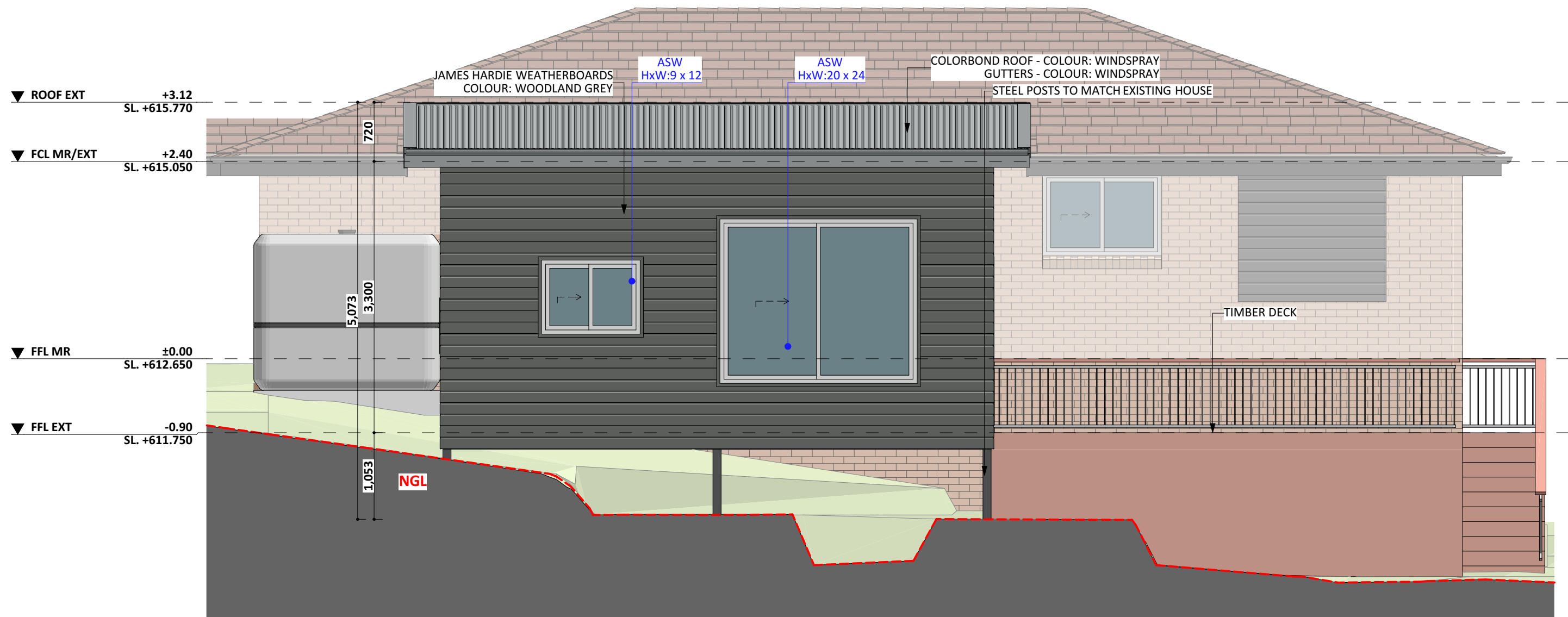
SOUTH ELEV.
