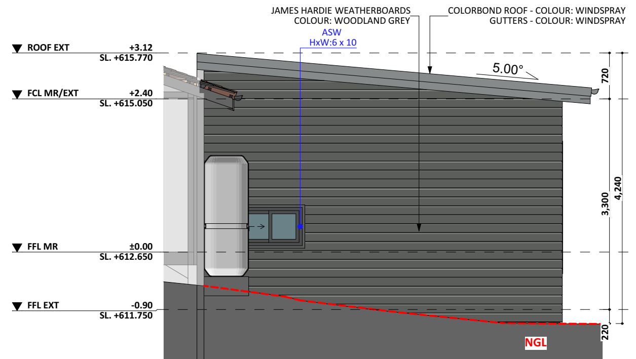
WEST ELEV.
