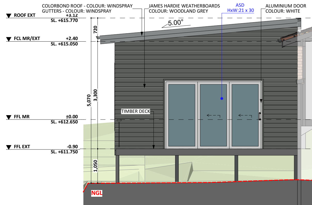
EAST ELEV.
