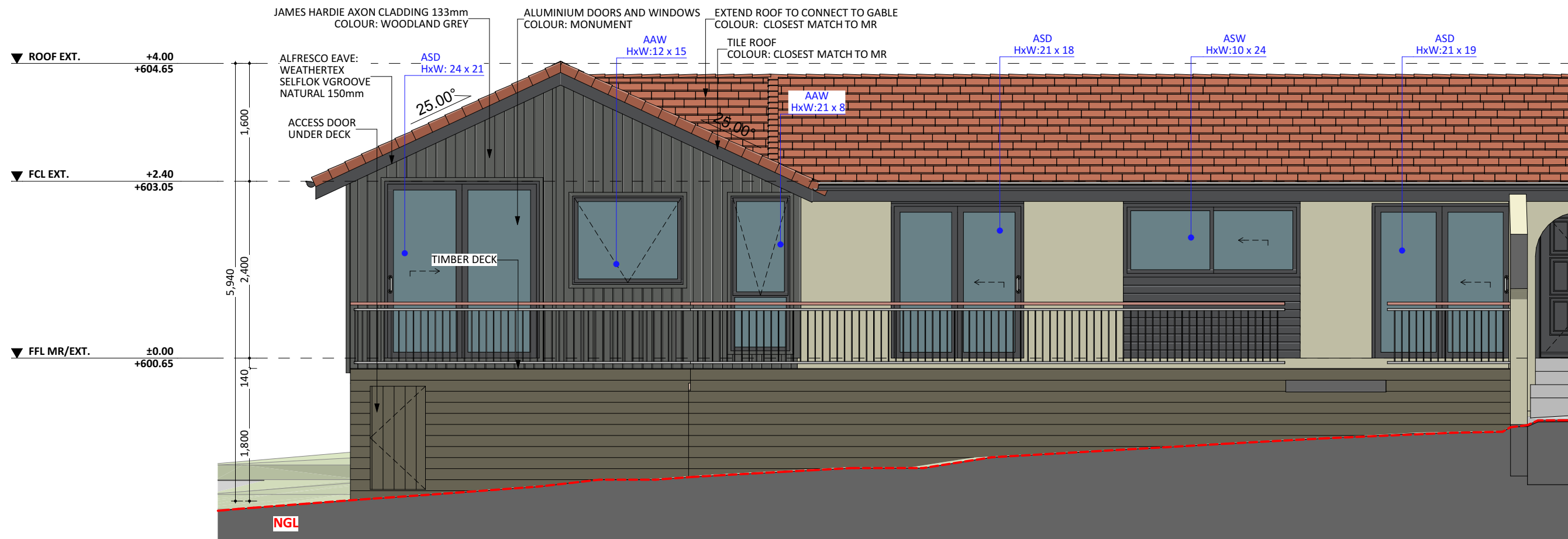
NORTH ELEV. - EXT.
