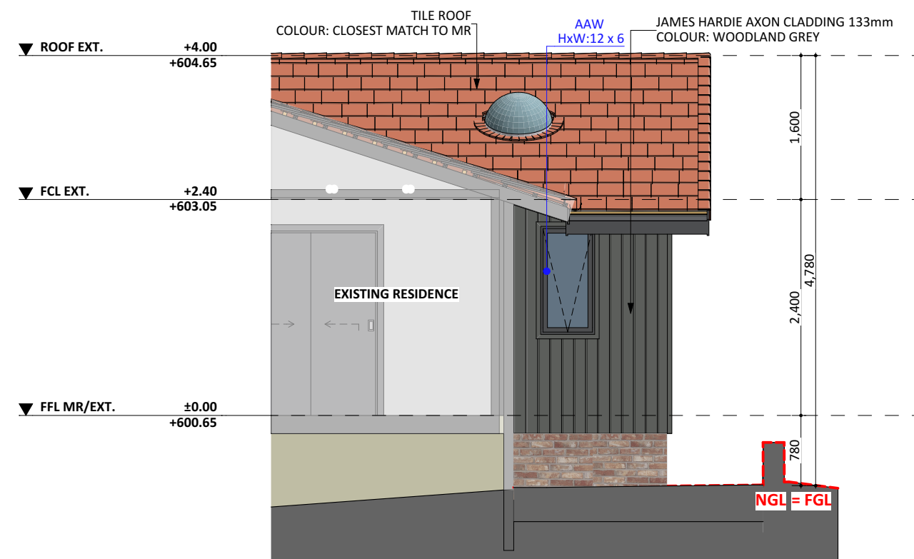
WEST ELEV. - EXT.
