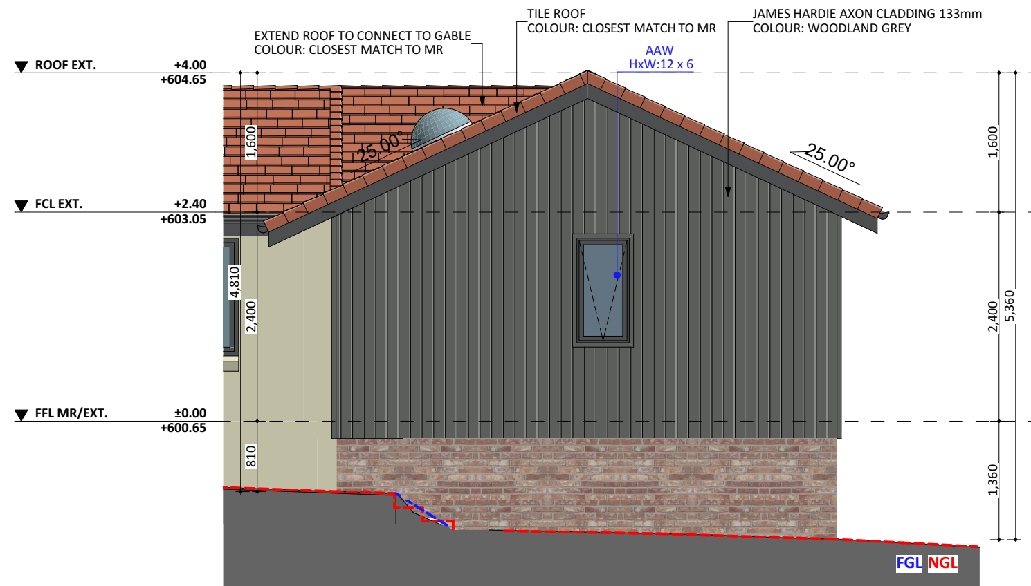
SOUTH ELEV. - EXT.
