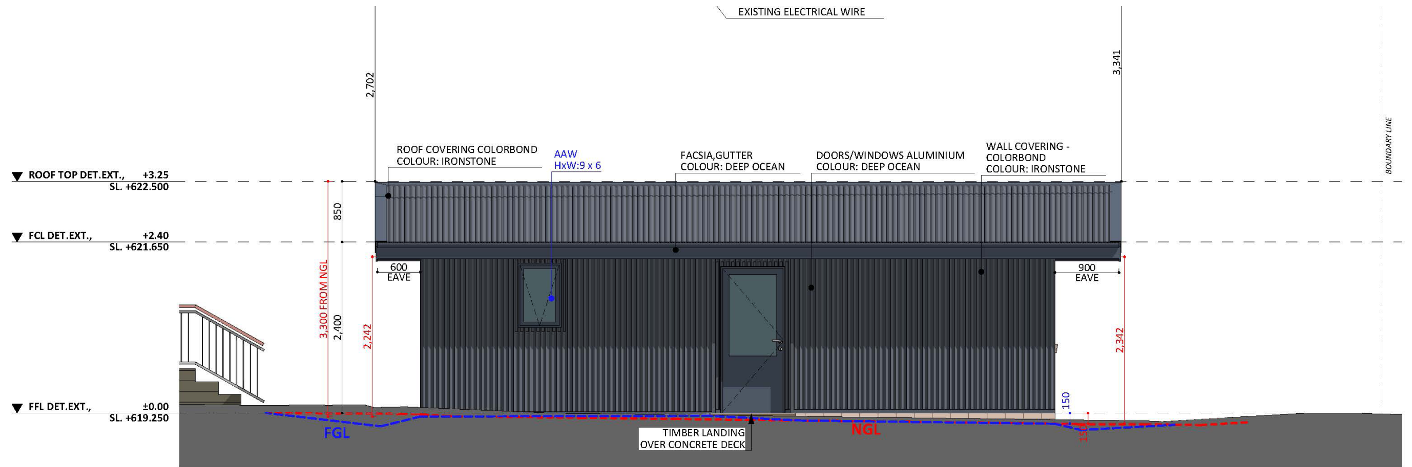
EAST ELEVATION 1:50
