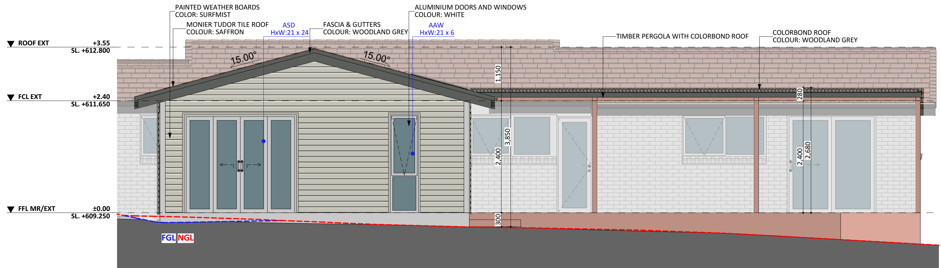
NORTH ELEV.
