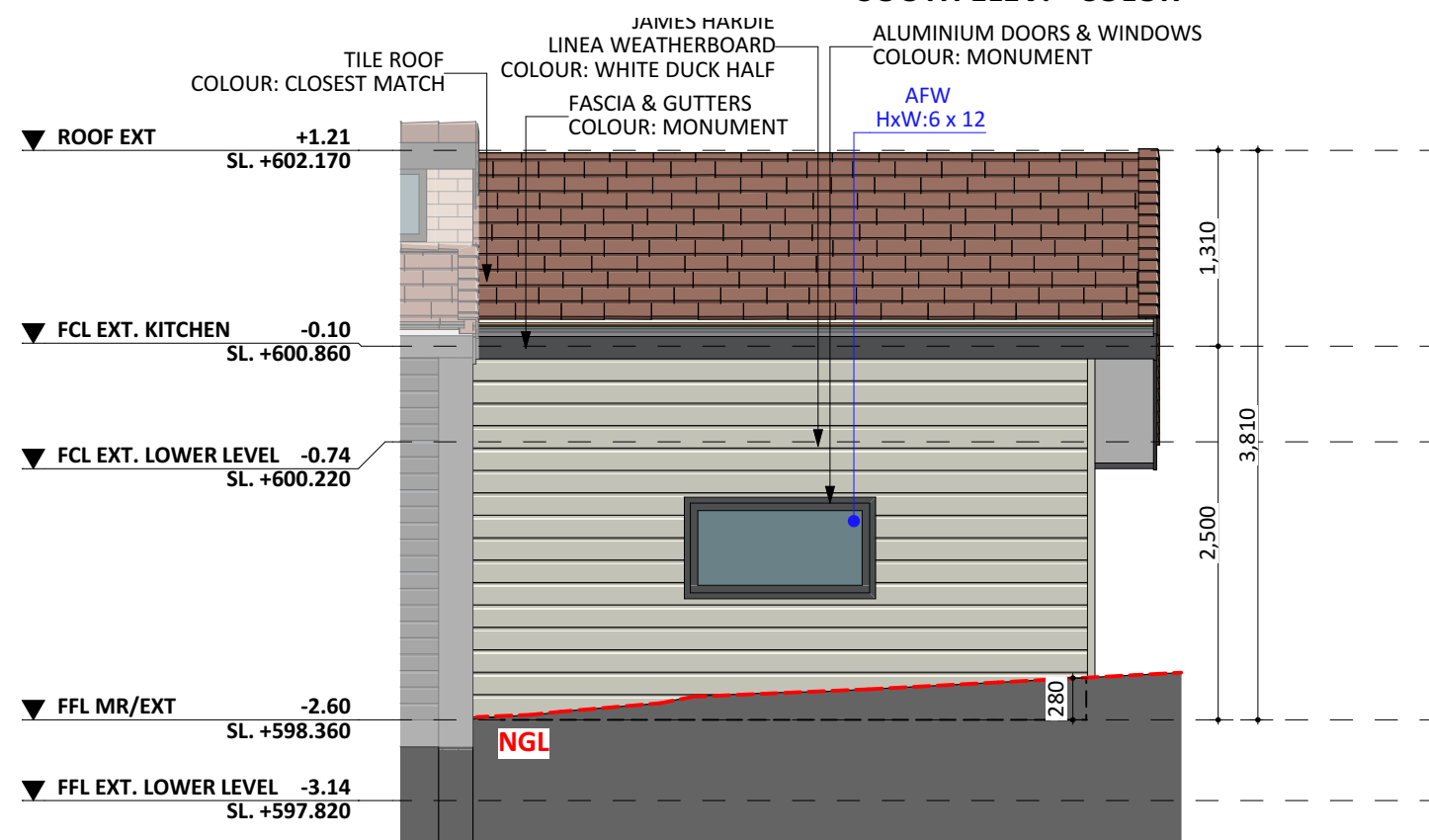
NORTH ELEV. - COLOR
