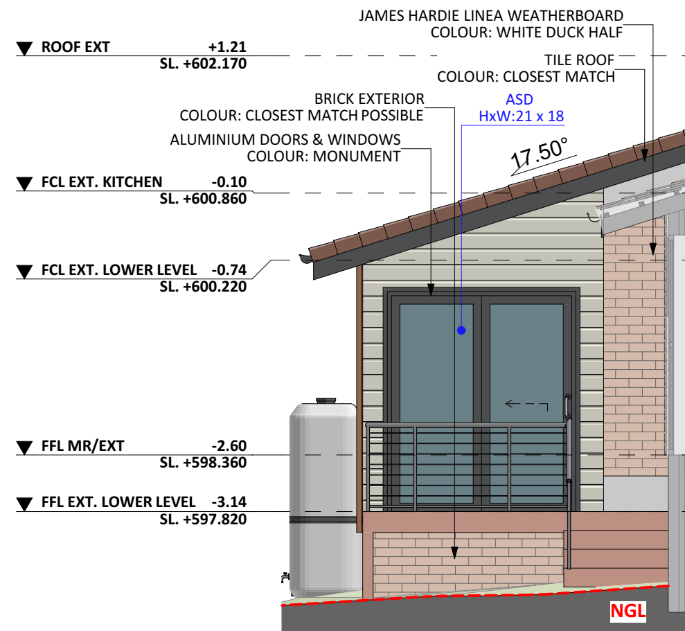
EAST ELEV. - COLOR
