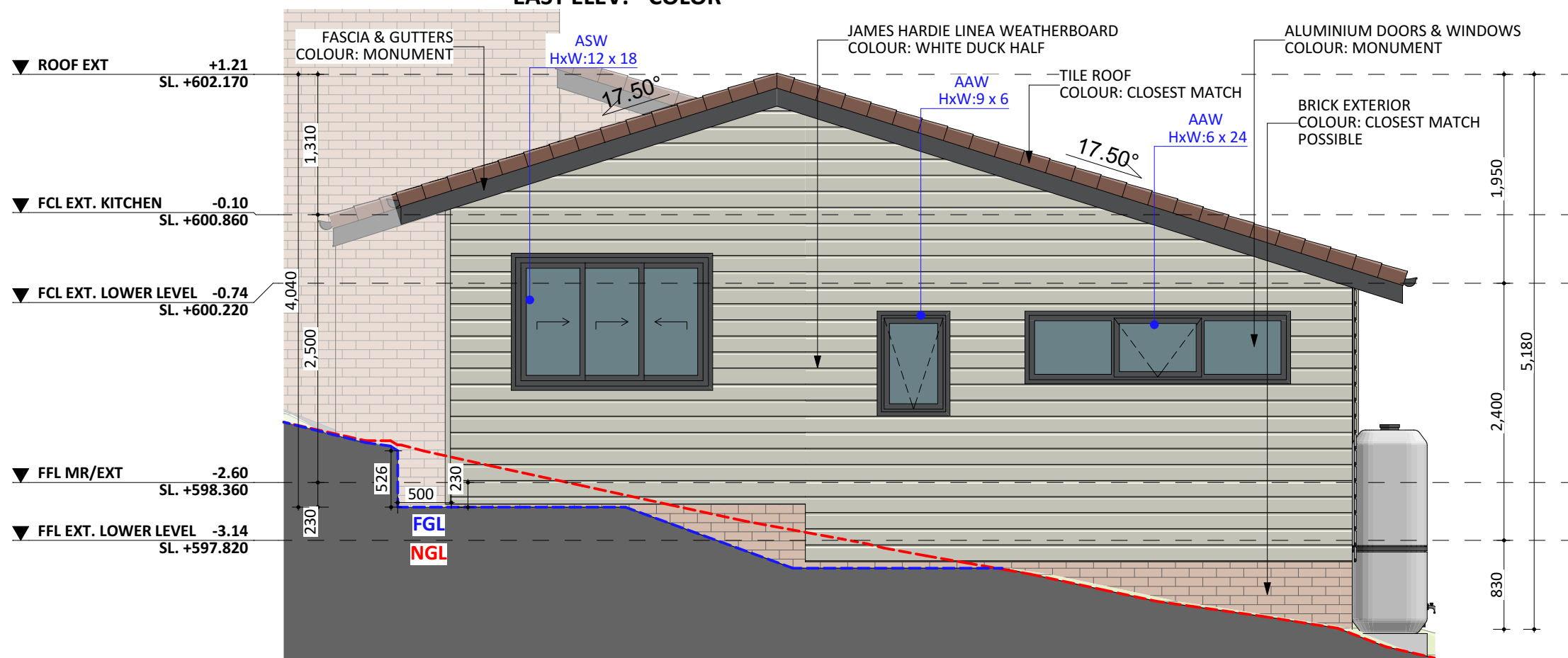
WEST ELEV. - COLOR
