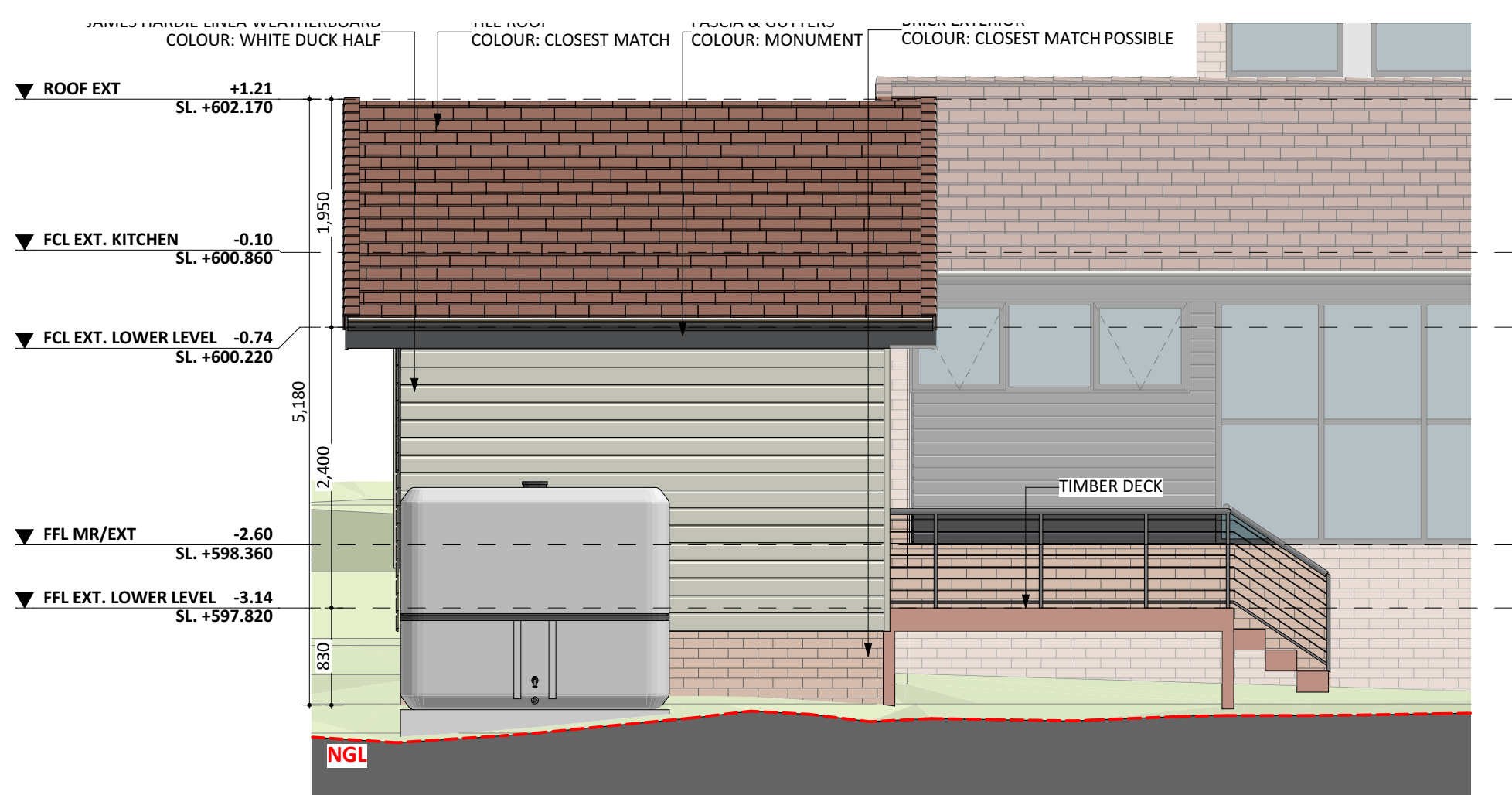
SOUTH ELEV. - COLOR
