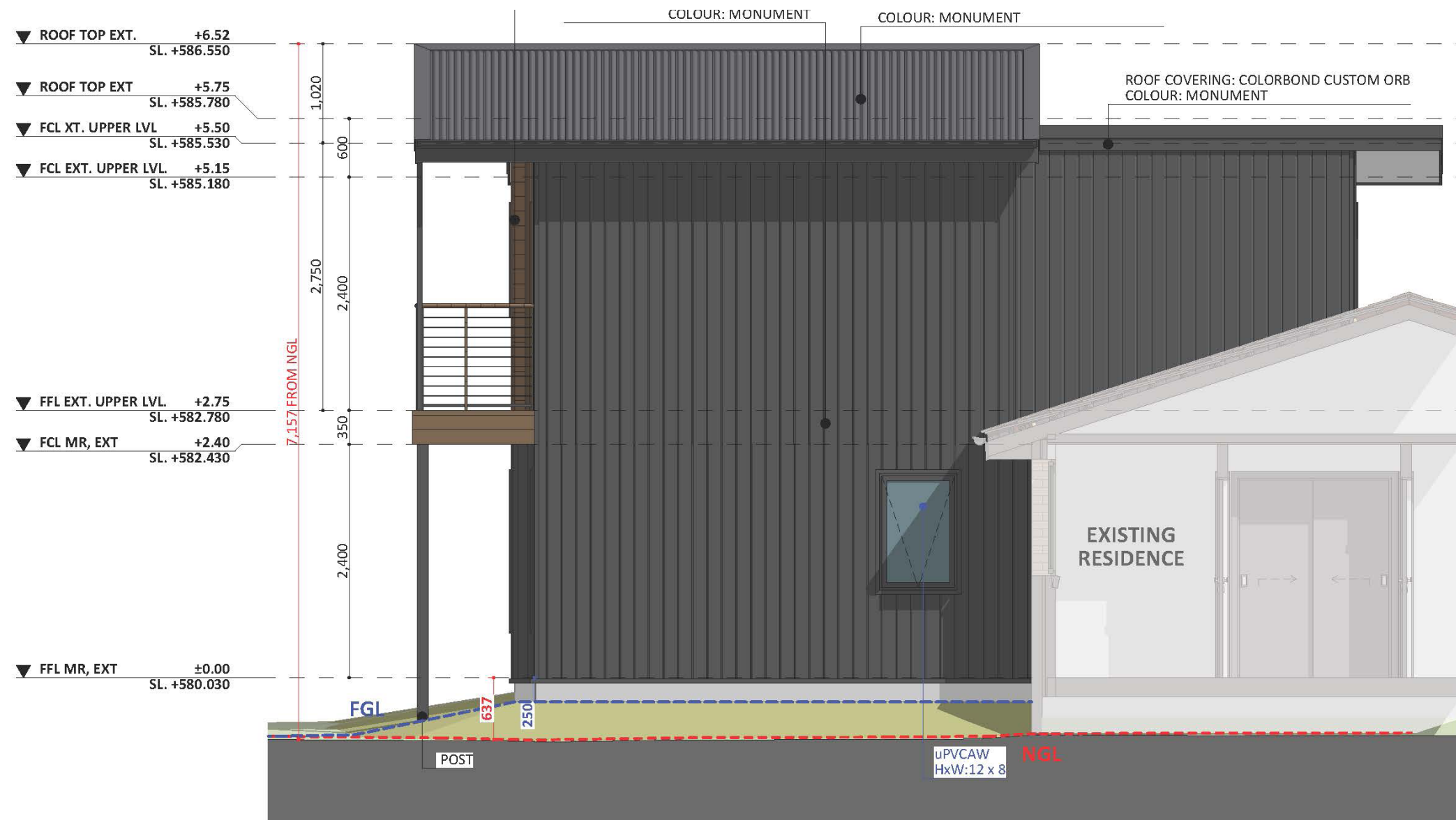
EAST ELEVATION
