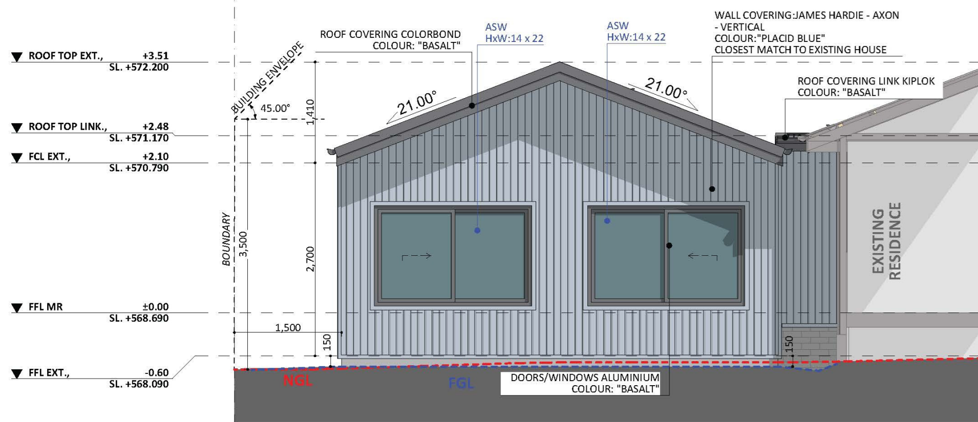
NORTH ELEVATION
