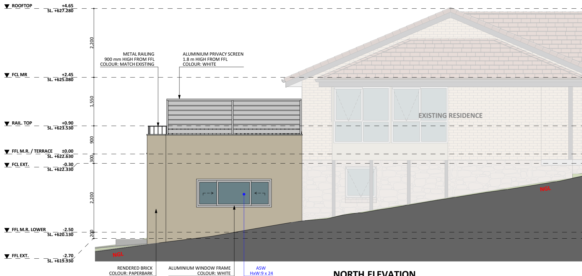
NORTH ELEVATION
