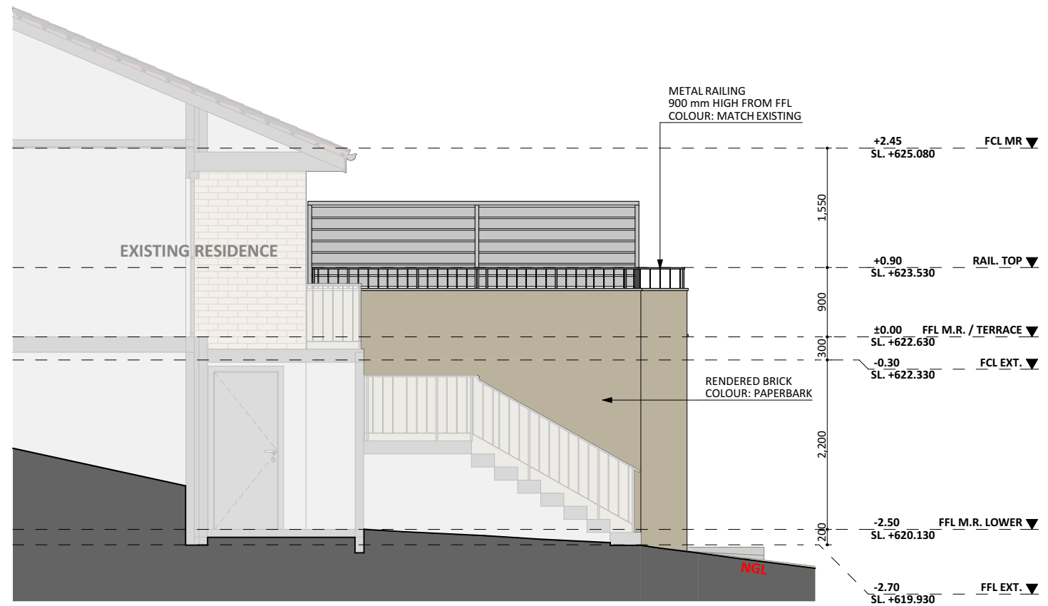
NORTH ELEVATION
