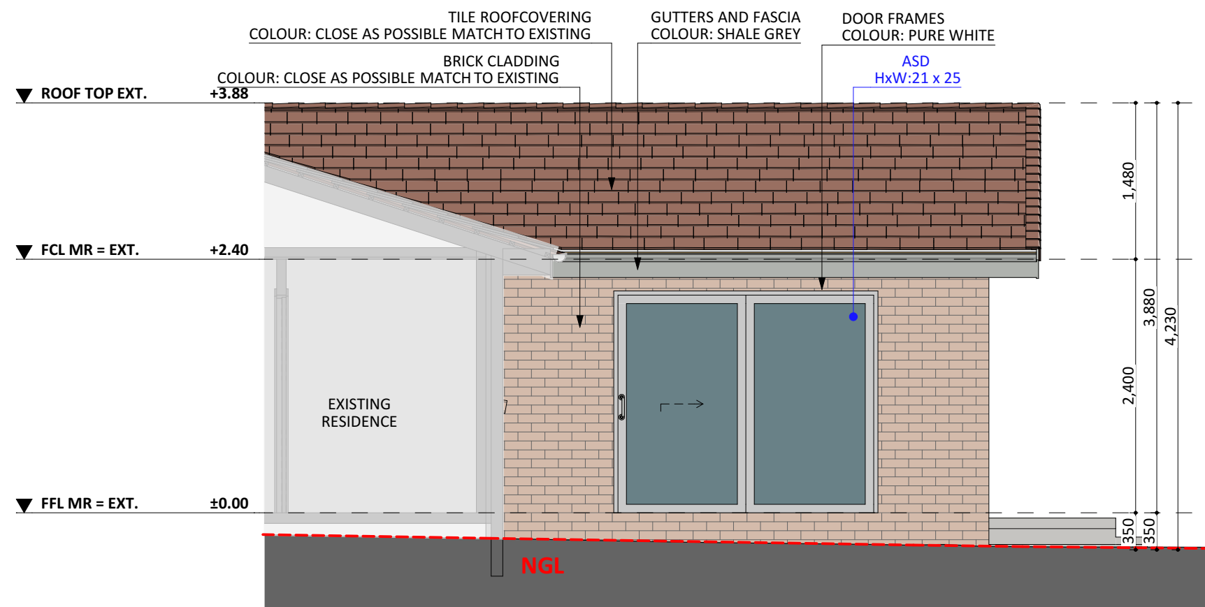
SOUTH-EAST ELEV. - EXT
