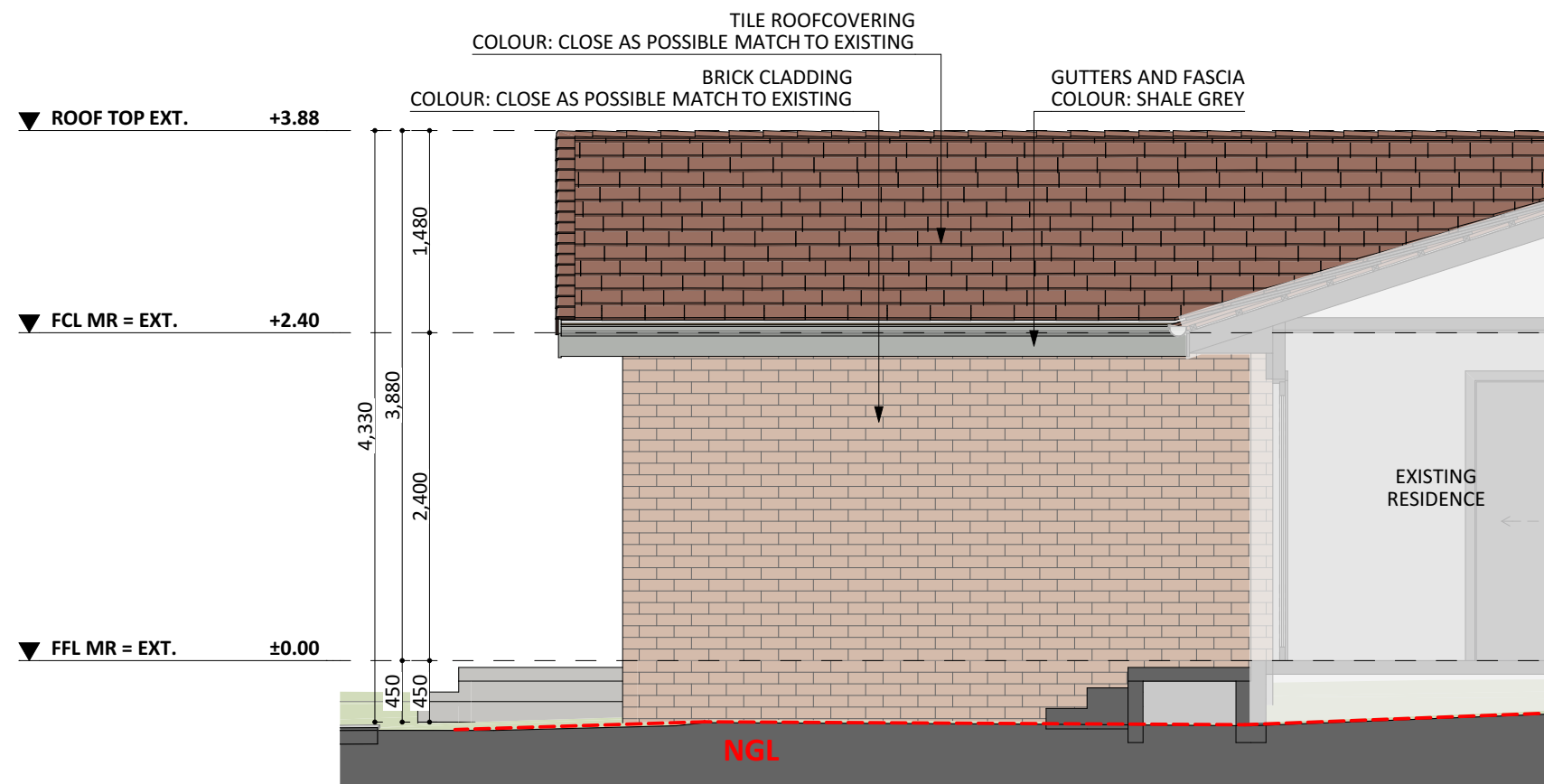
NORTH-WEST ELEV. - EXT.
