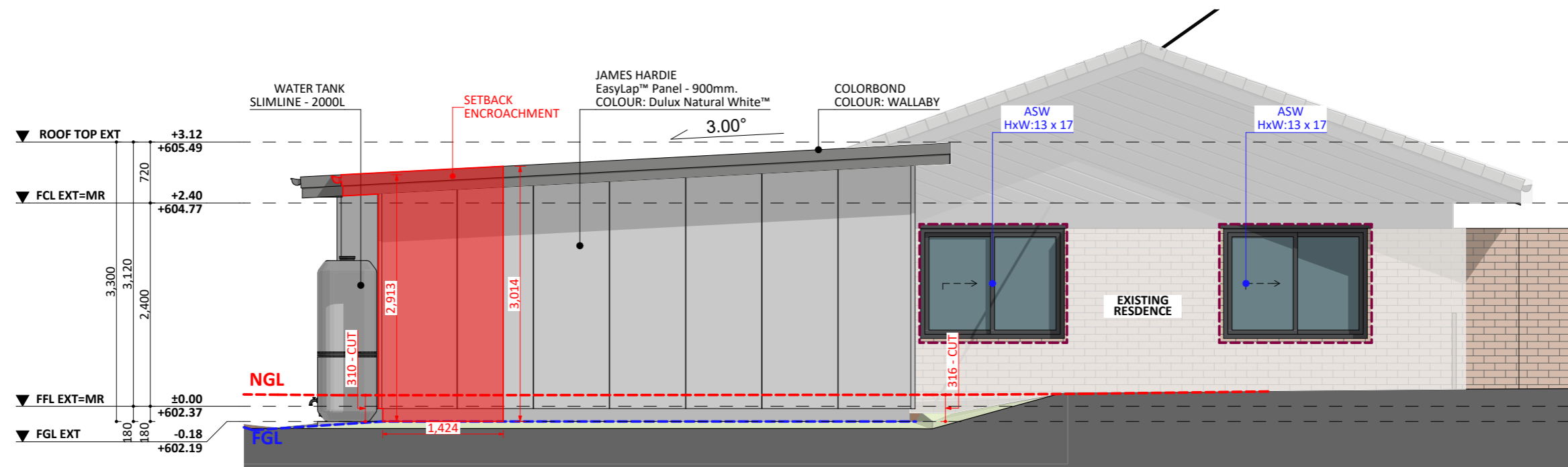
NORTH ELEV.
