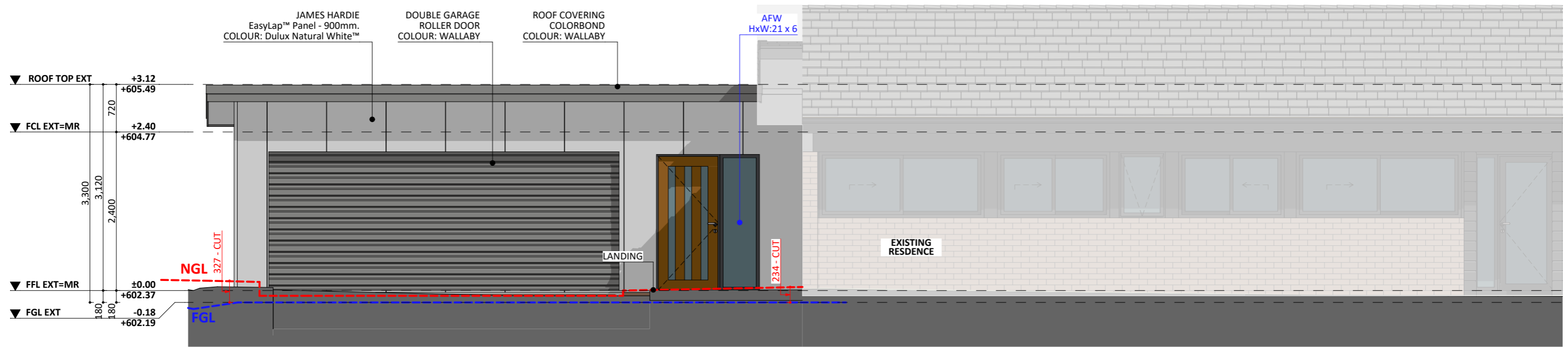
WEST ELEV.
