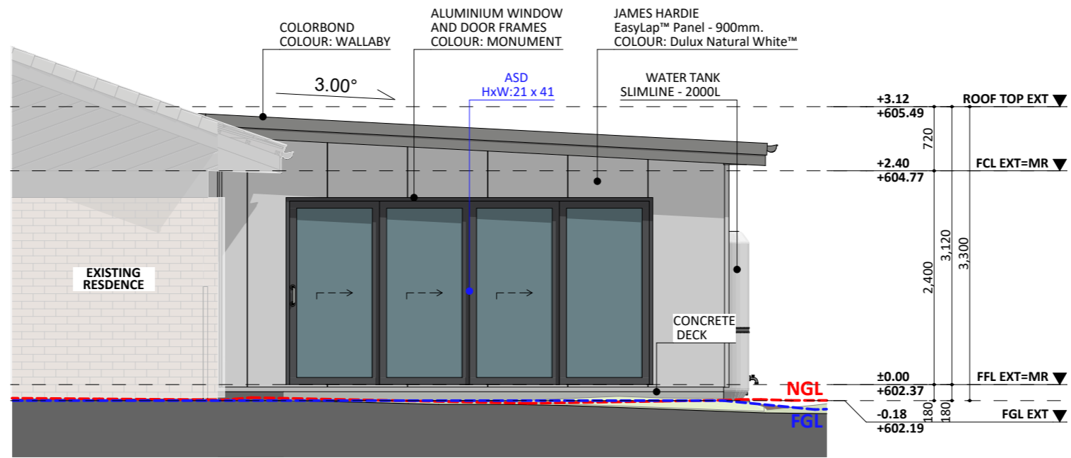
SOUTH ELEV.
