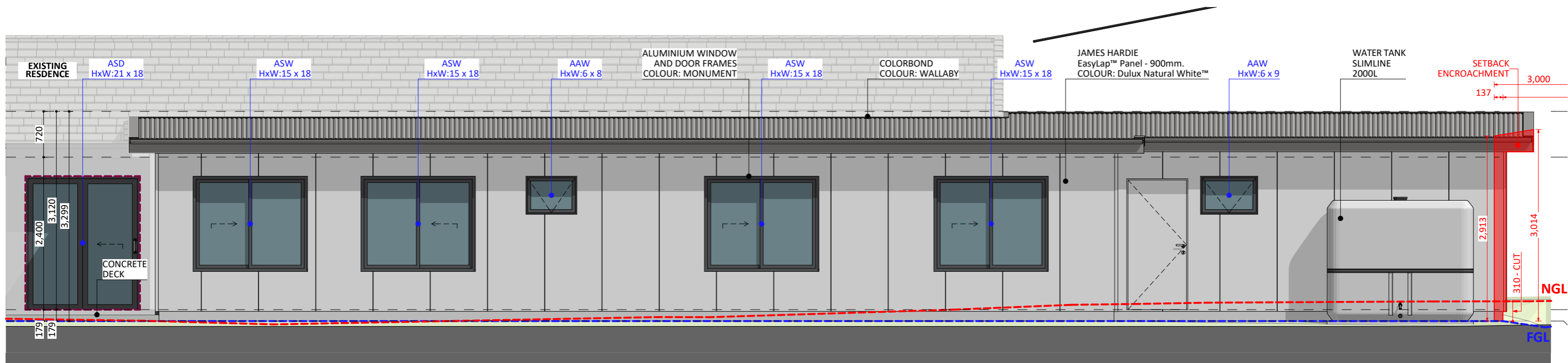
EAST ELEV.
