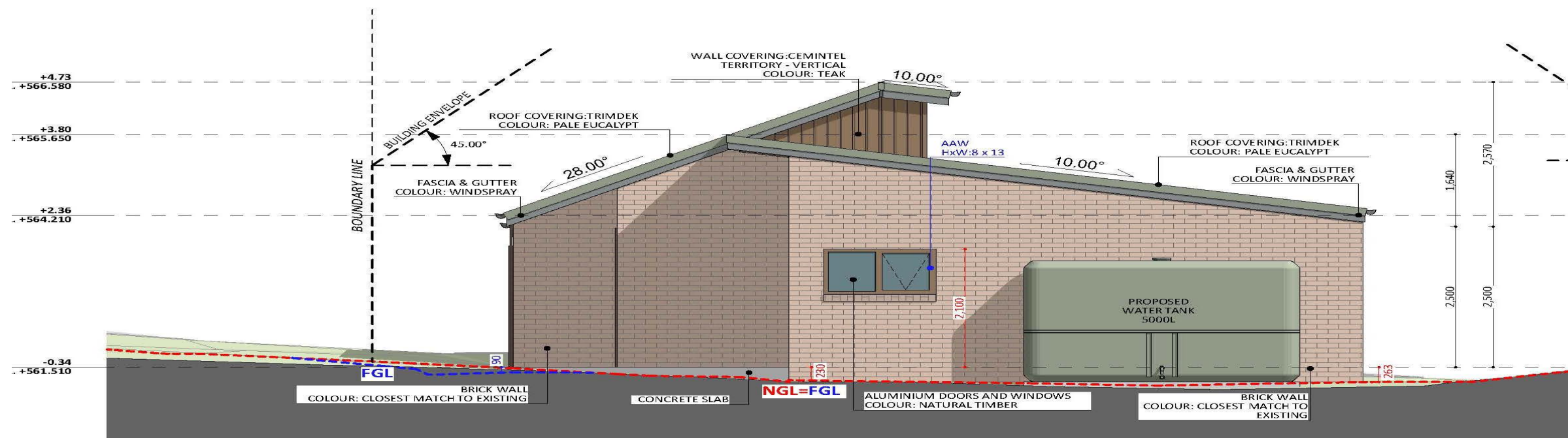
EAST ELEVATION
