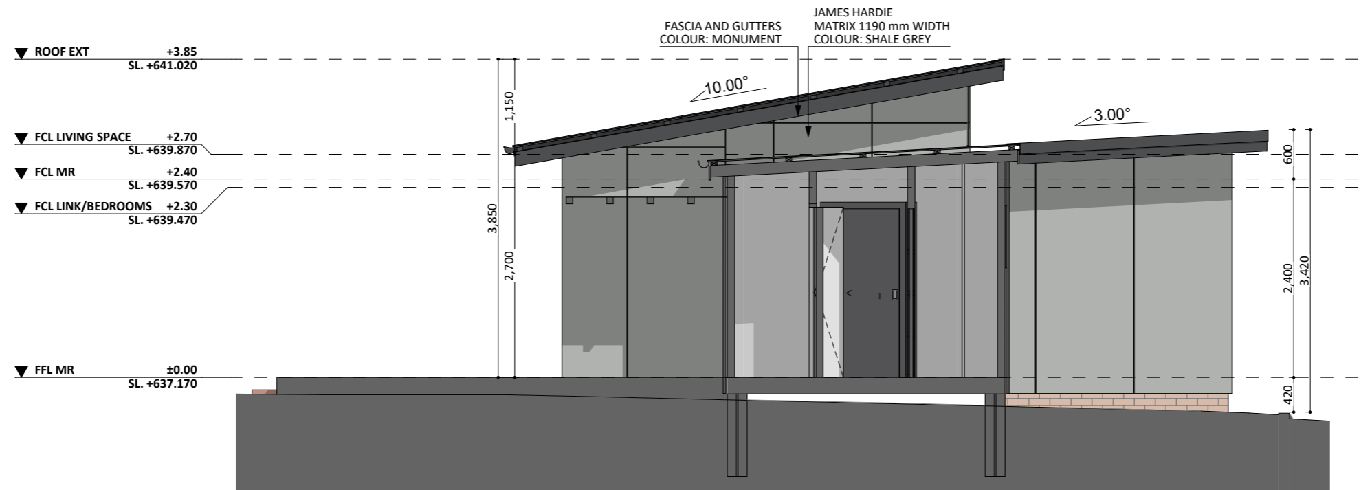
EAST ELEV
