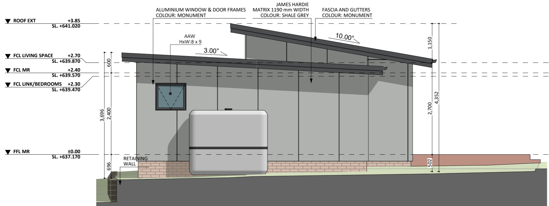
WEST ELEV.
