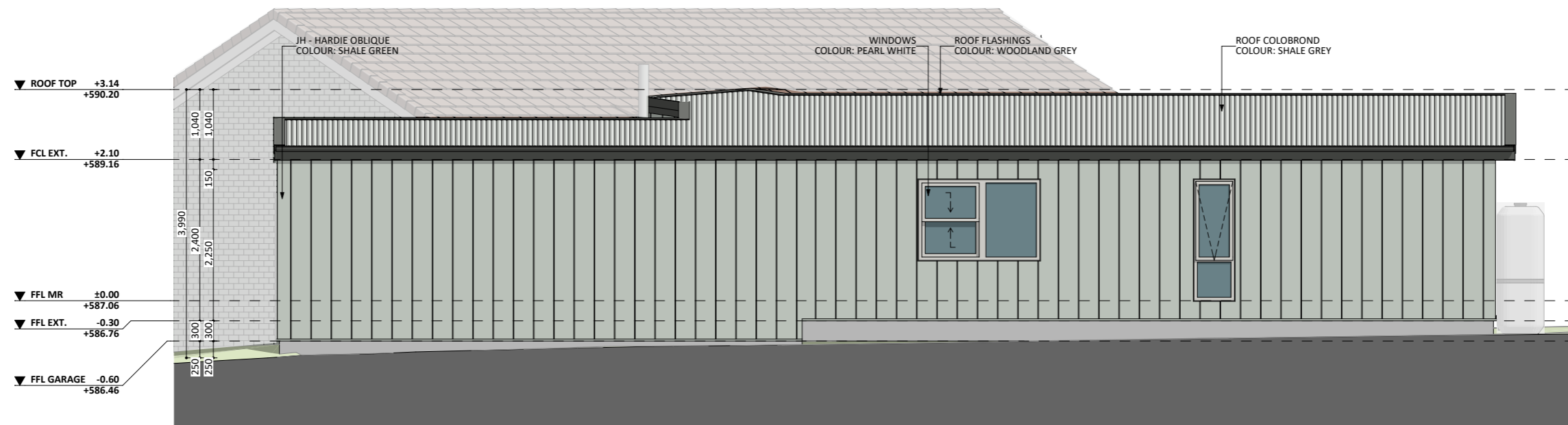
SOUTH-WEST ELEV.
