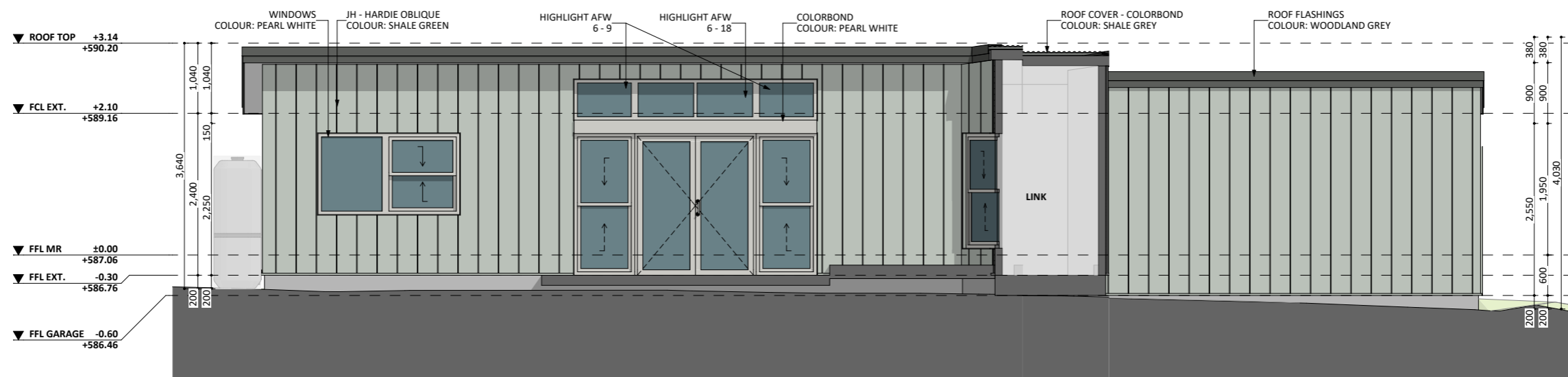
CD-E3 NORTH-EAST ELEV.
