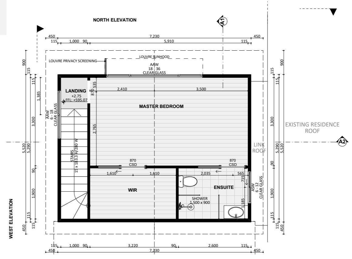
FIRST FLOOR
