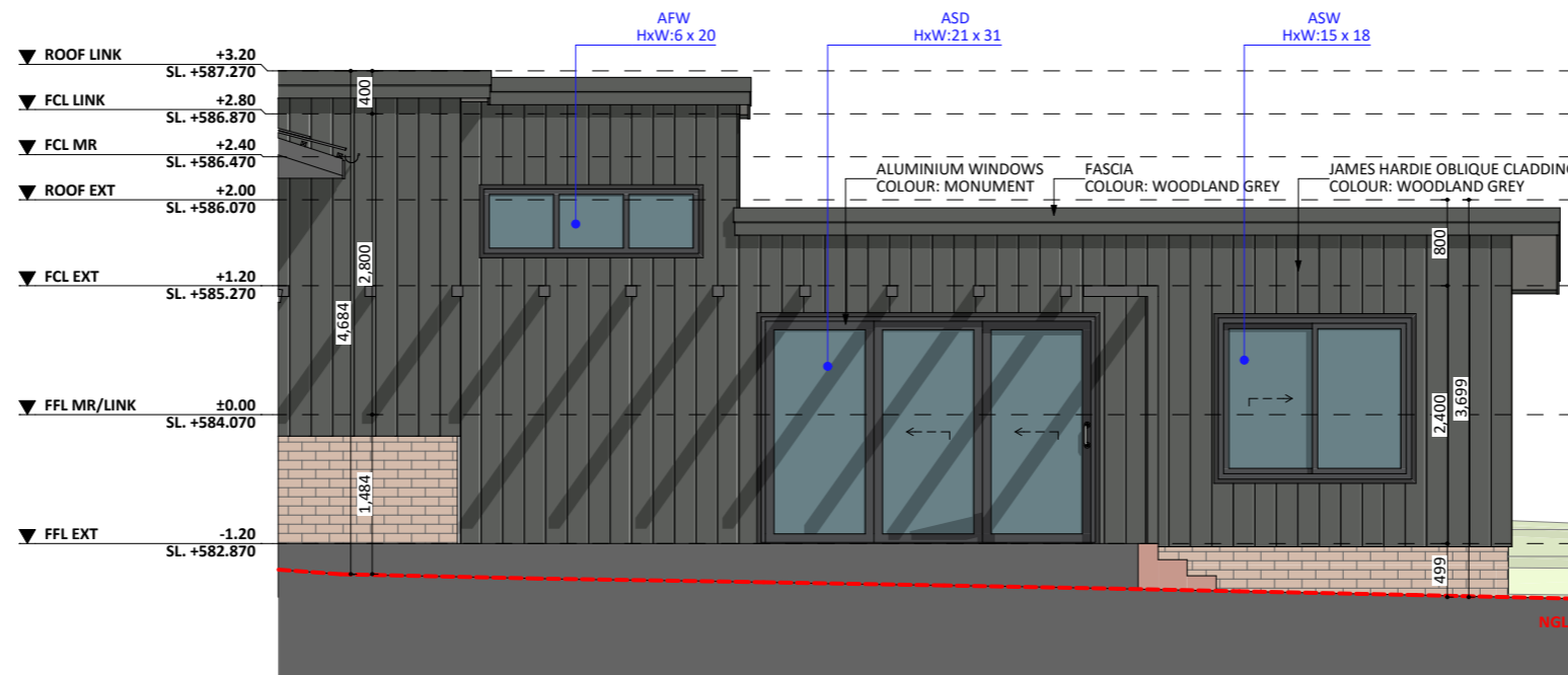
NORTH ELEV.
