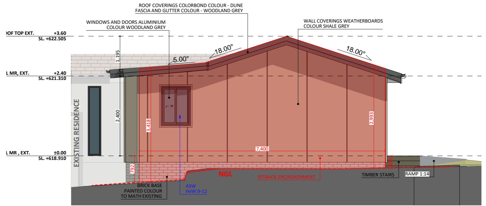
SOUTH - EAST ELEVATION - CL 1168
