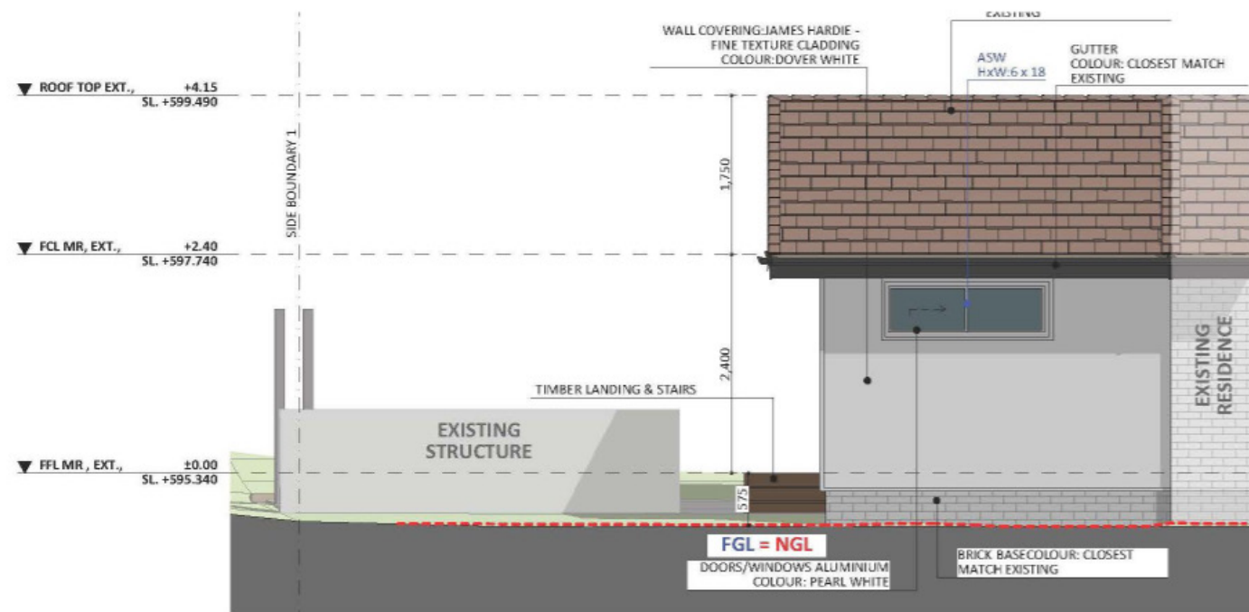
WEST ELEVATION
