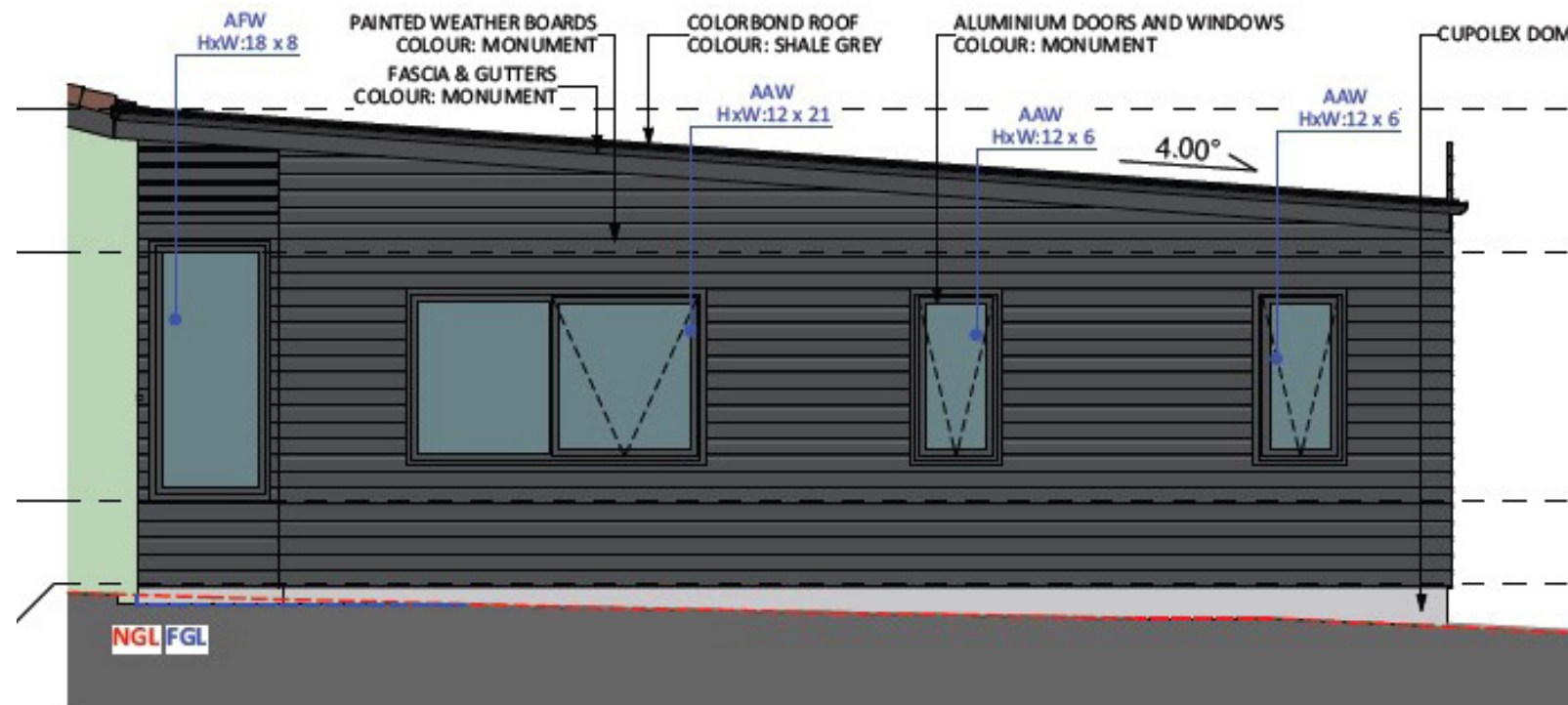
NORTH-WEST ELEV.
