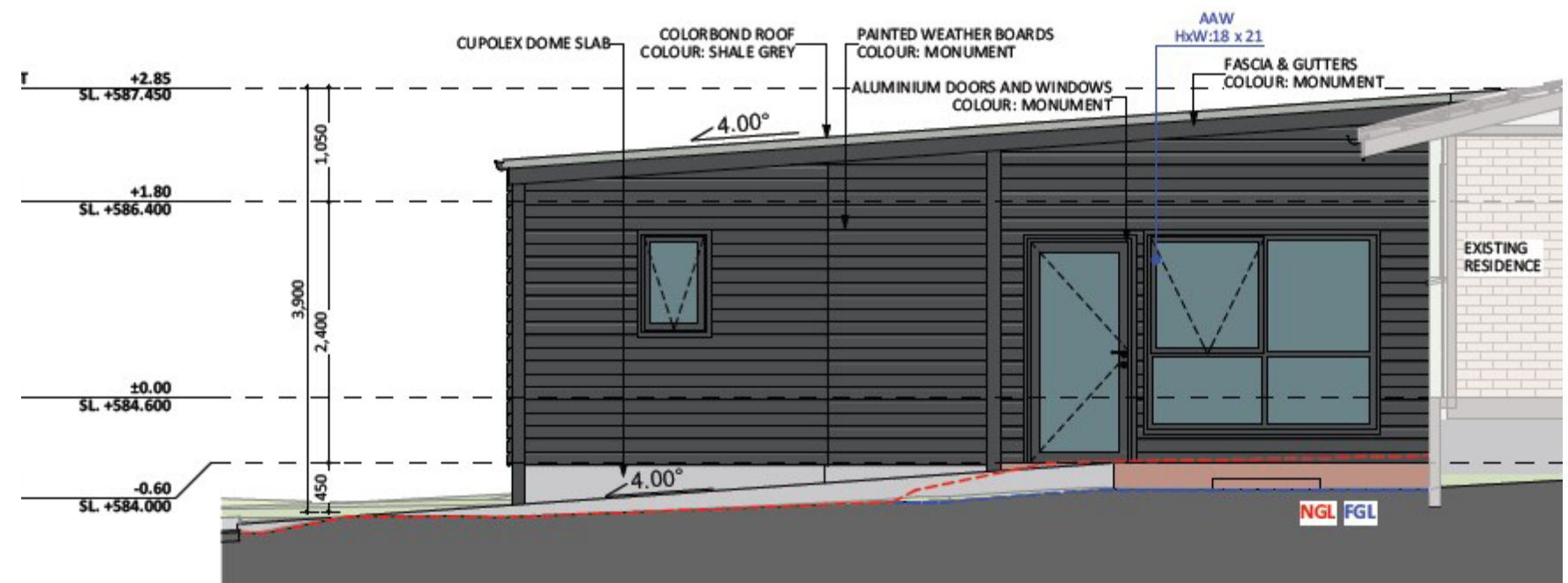
SOUTH-EAST ELEV.
