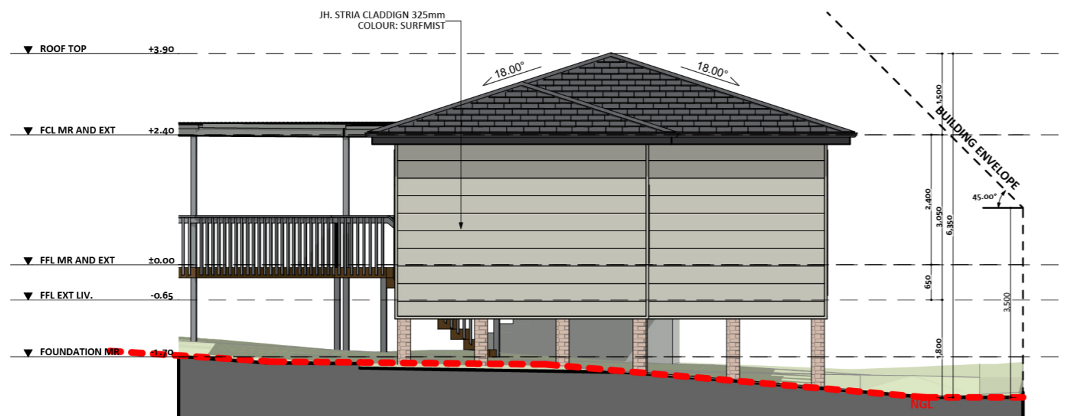
NORTH ELEVATION - CD
