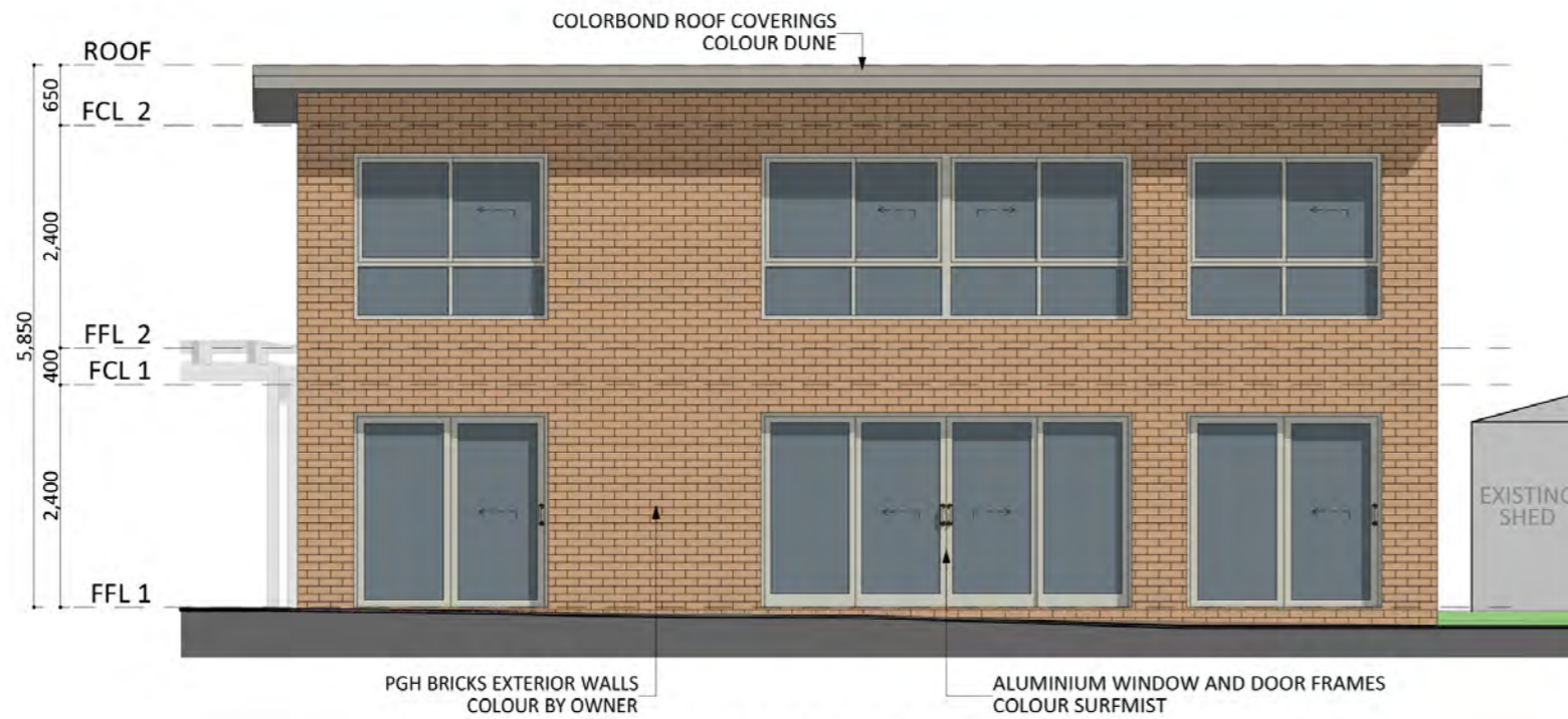
NORTH ELEVATION
