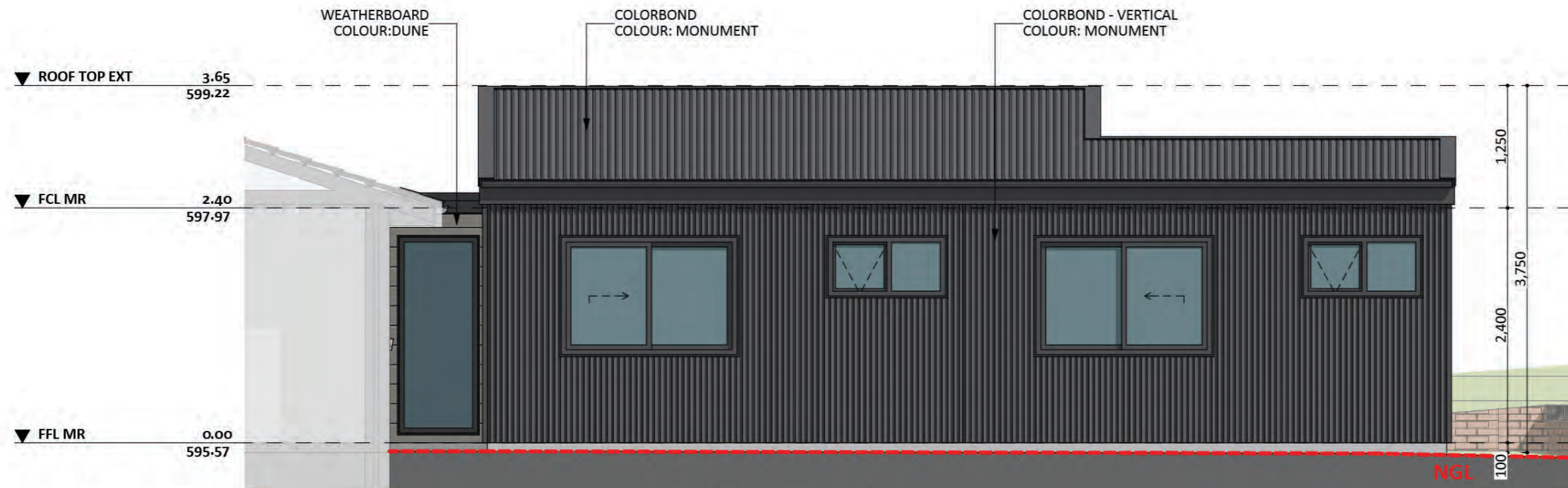
SOUTH-WEST ELEVATION
