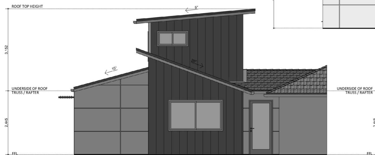
ELEVATION 03
