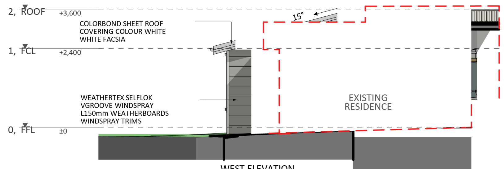
WEST ELEVATION
