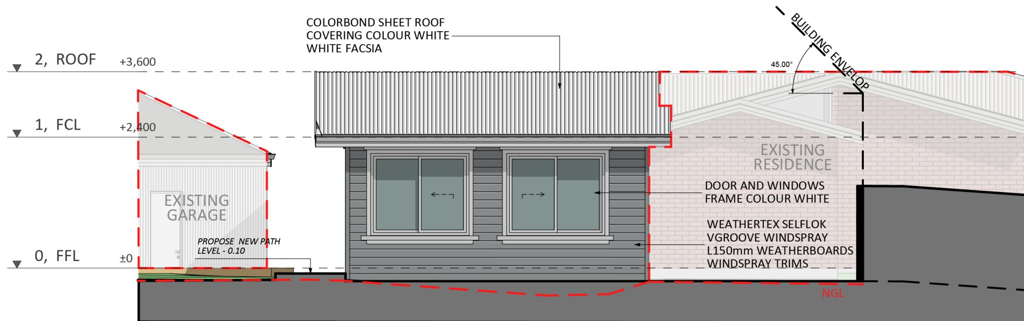
NORTH ELEVATION
