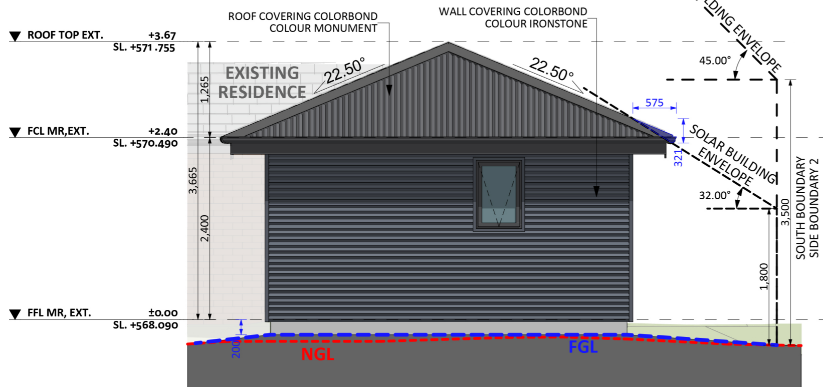
ELEVATION 03
