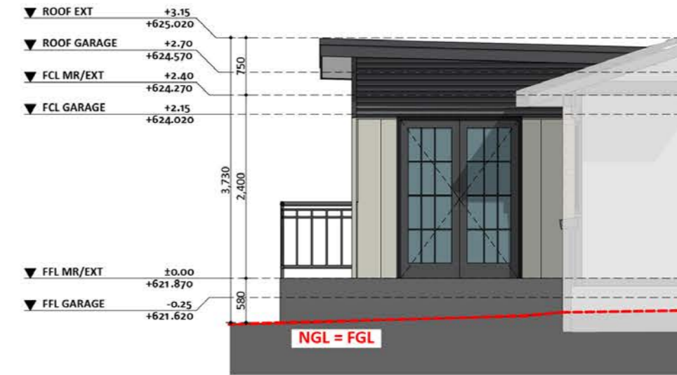
SOUTH-EAST ELEVATION
