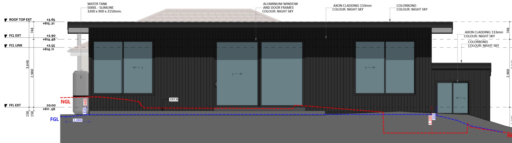
ELEVATION 03
