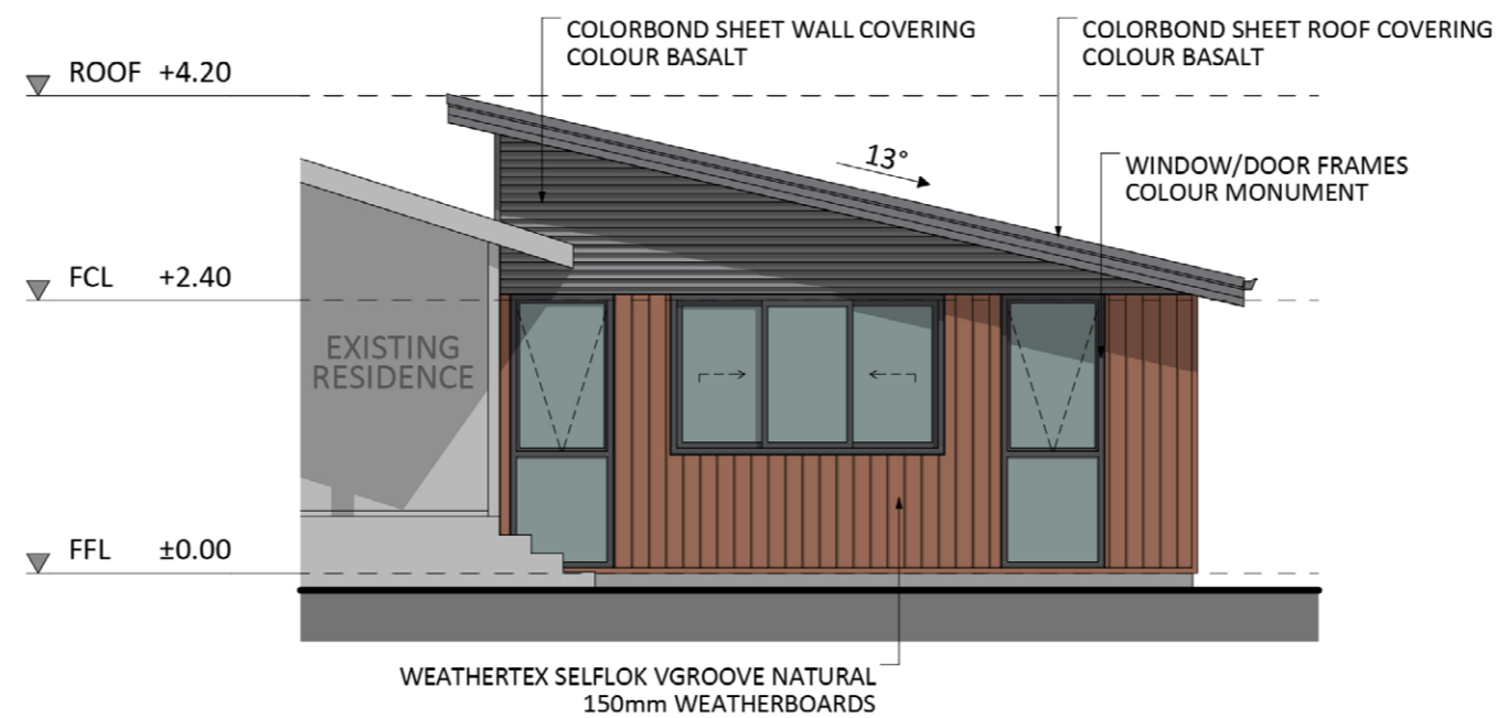
WEST ELEVATION
