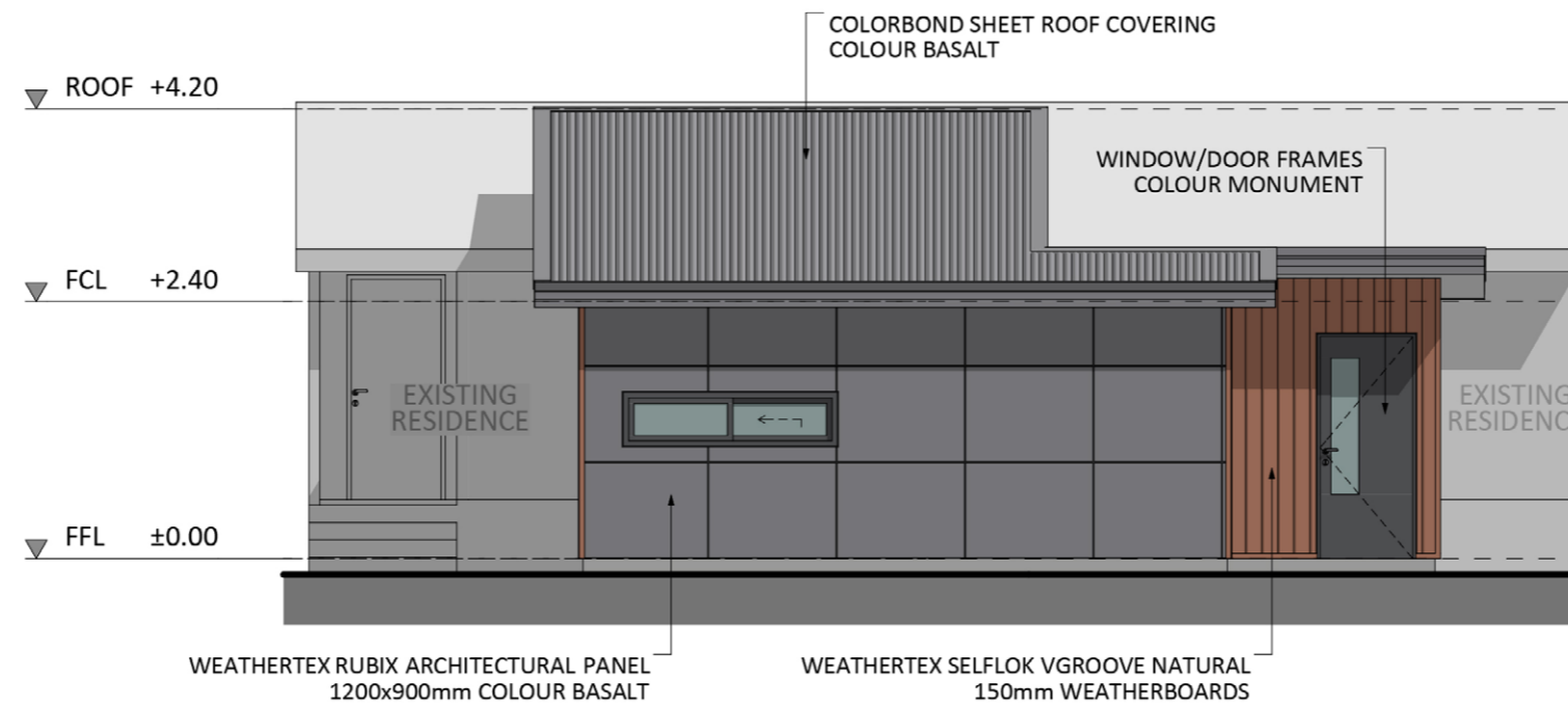
SOUTH ELEVATION
