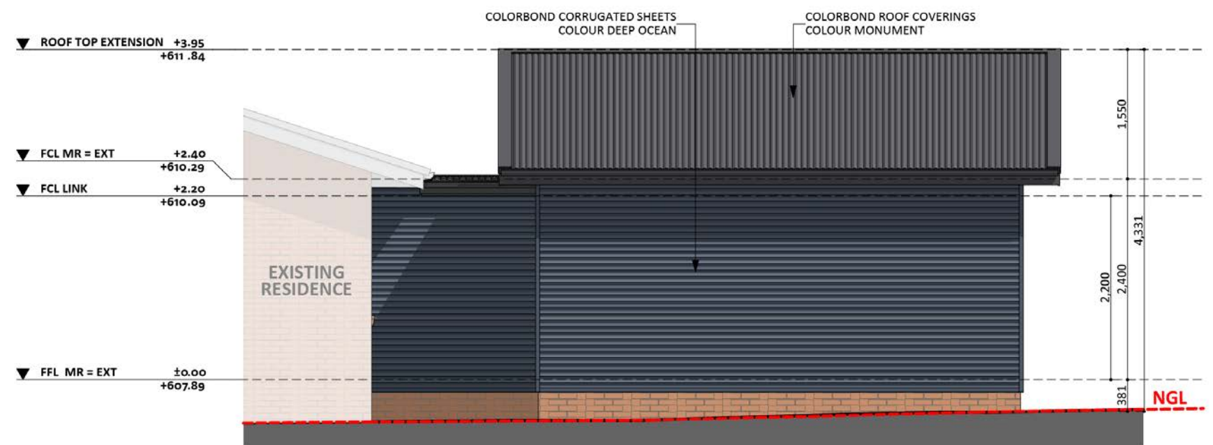
NORTH-WEST ELEVATION
