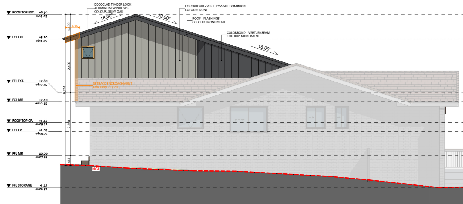
NORTH-WEST ELEVATIONS
