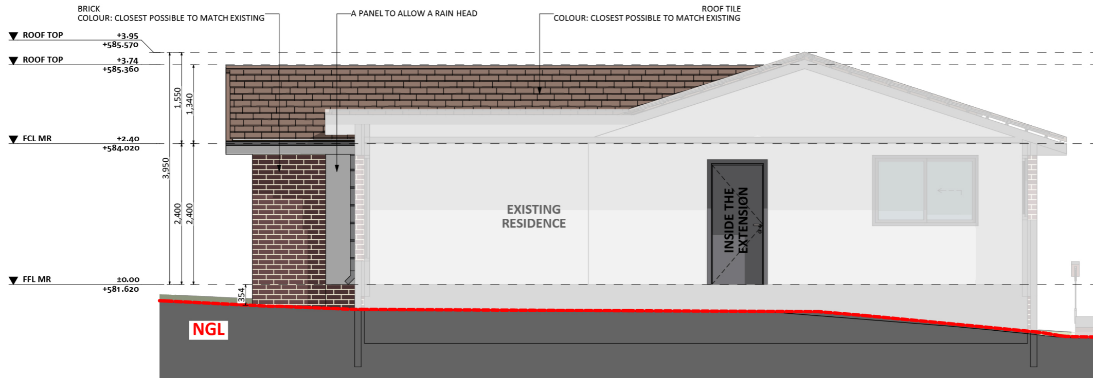
ELEVATION 03
