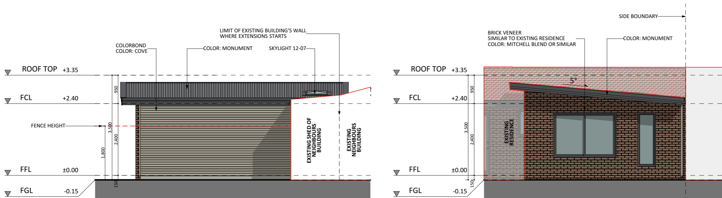
NORTH-EAST ELEVATION - OPT 2
