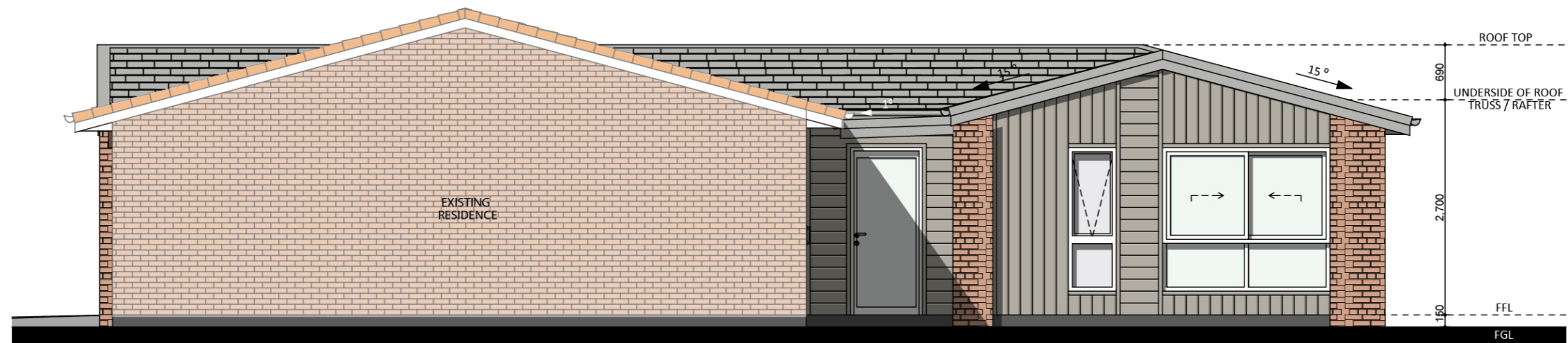
EAST ELEVATION
