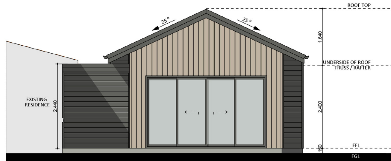
NORTH ELEVATION
