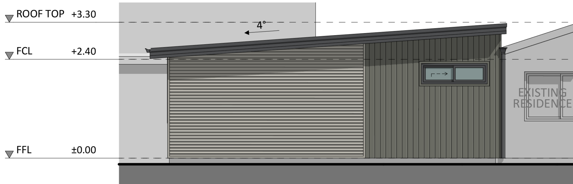
NORTH-WEST ELEVATION
