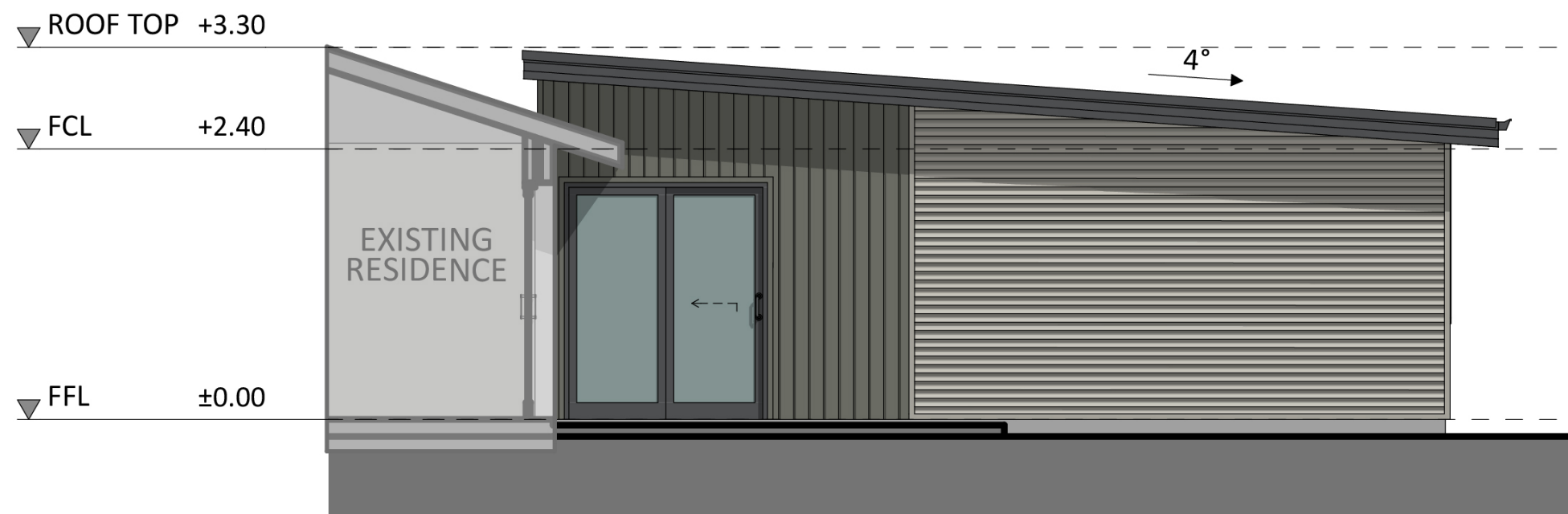
SOUTH-EAST ELEVATION
