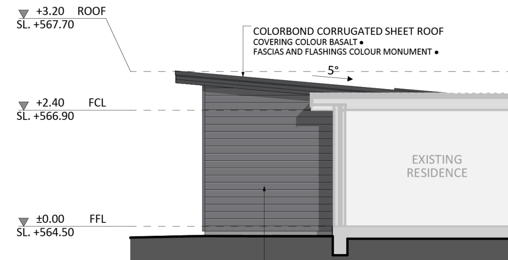
WEST ELEVATION
