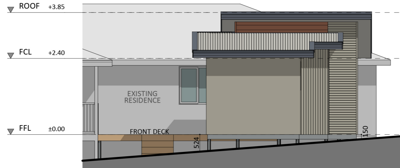
NORTH-WEST ELEVATION
