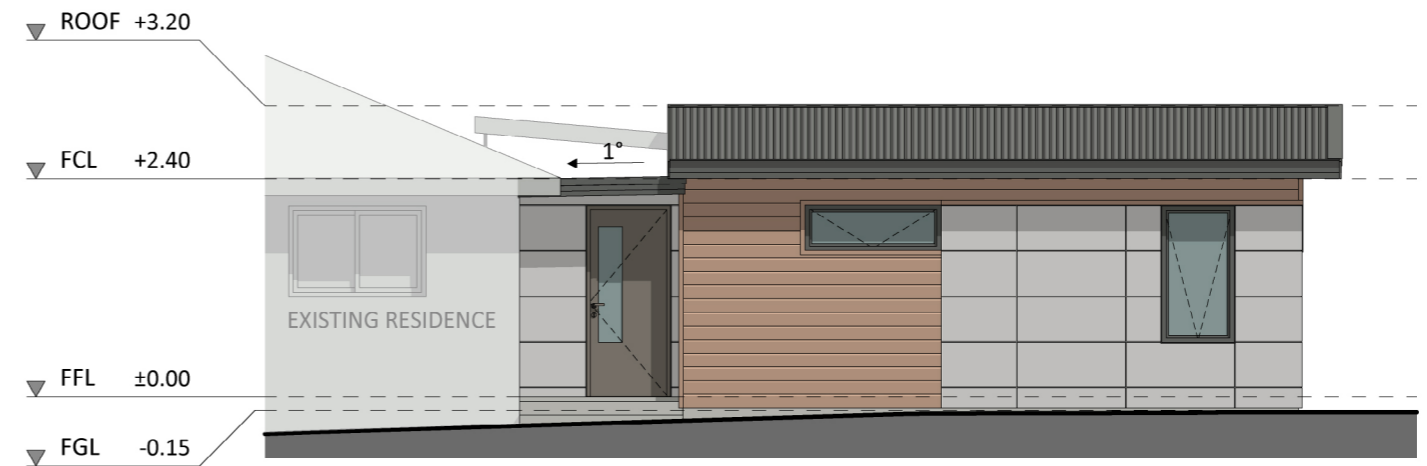
NORTH-WEST ELEVATION
