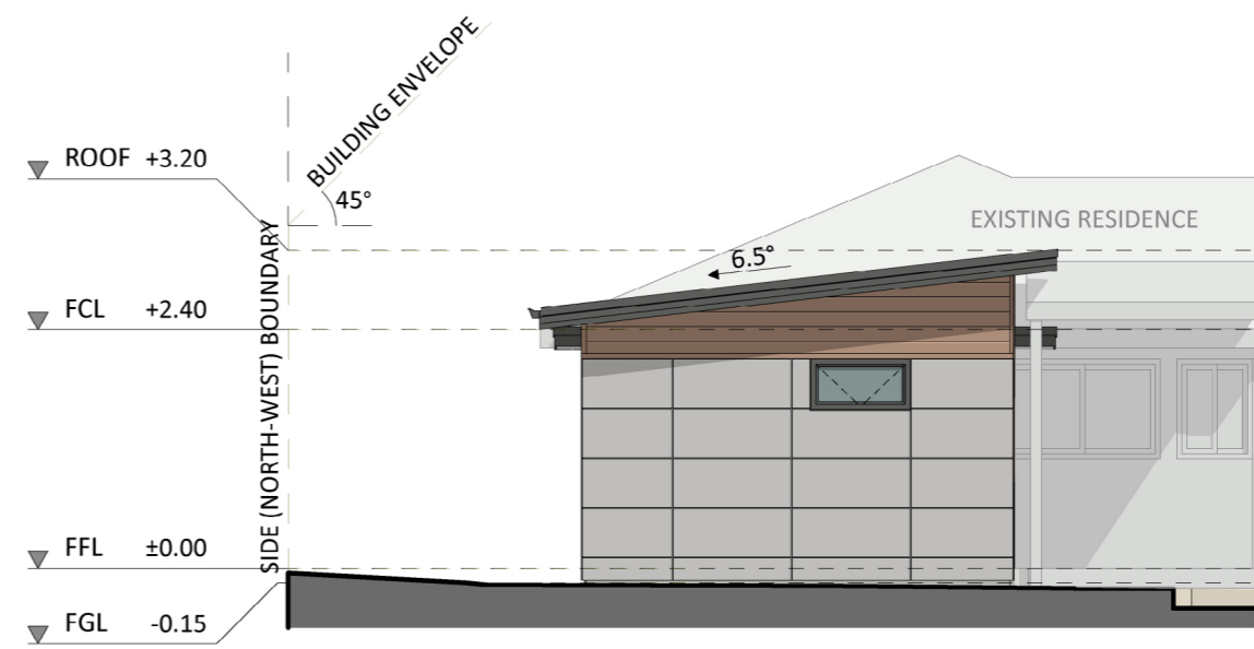
SOUTH-WEST ELEVATION
