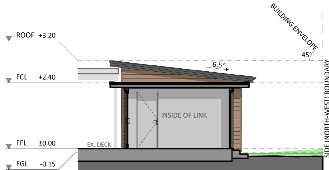
NORTH-EAST ELEVATION
