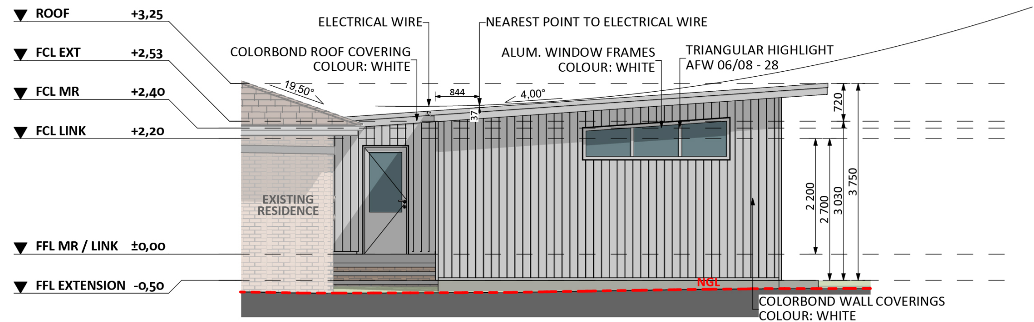
EAST ELEVATION
