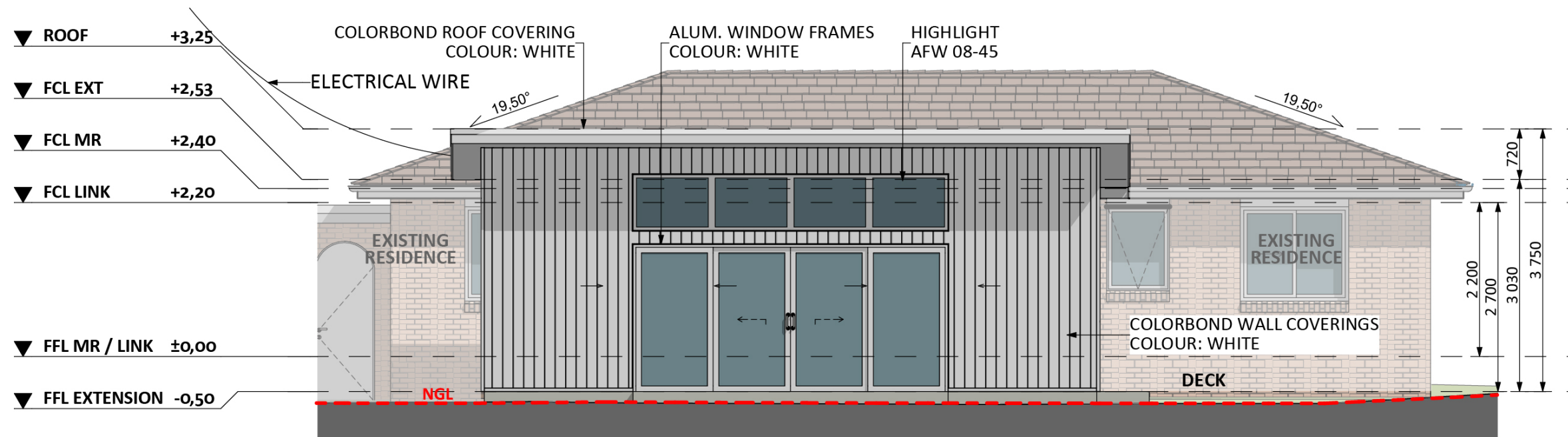
NORTH ELEVATION
