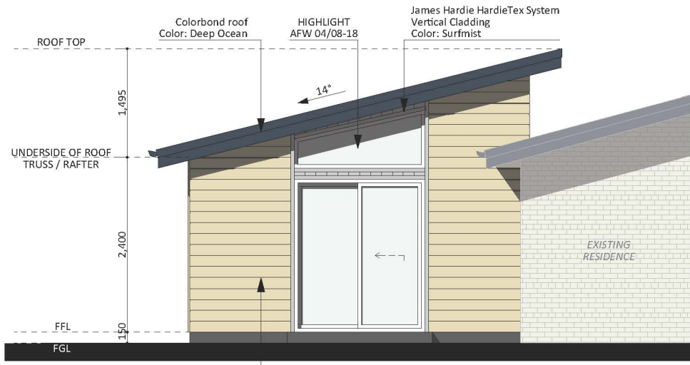
NORTH-EAST ELEVATION
