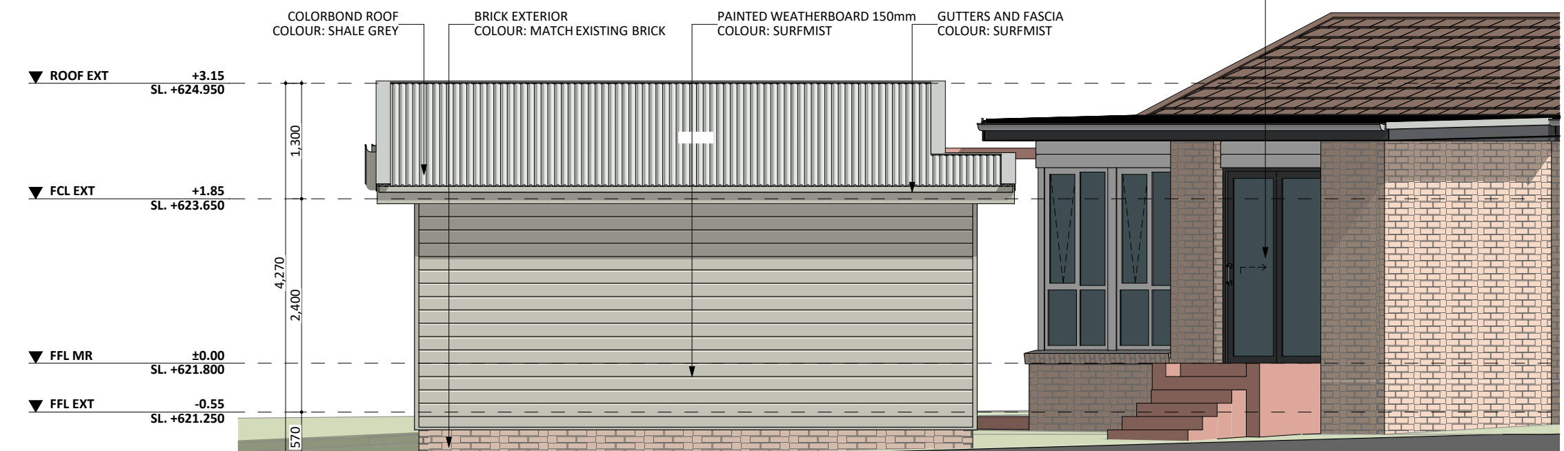
WEST ELEV.
