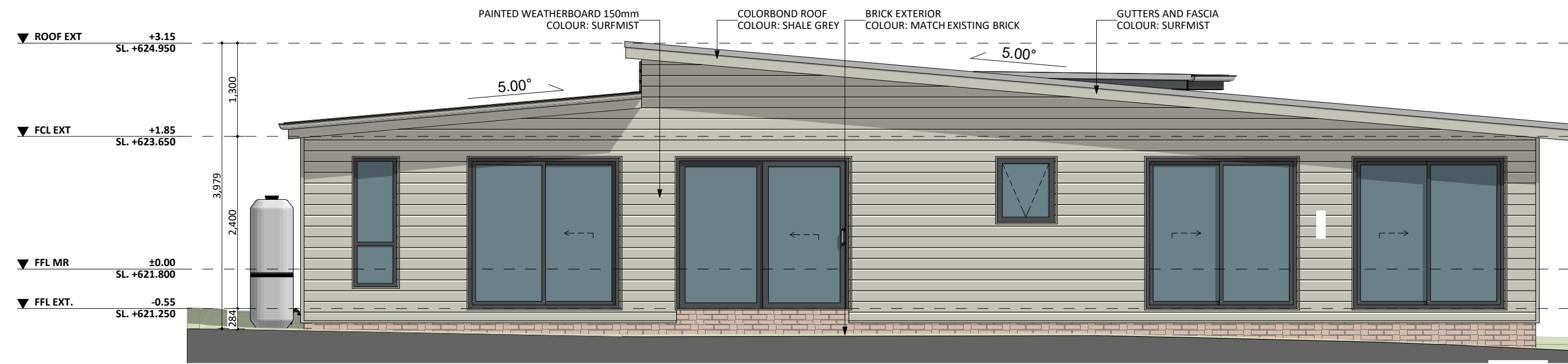
NORTH ELEV.
