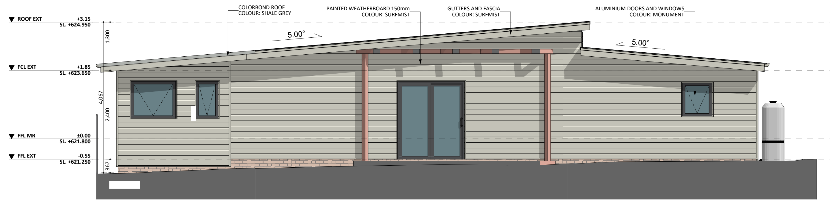
SOUTH-WEST ELEV.
